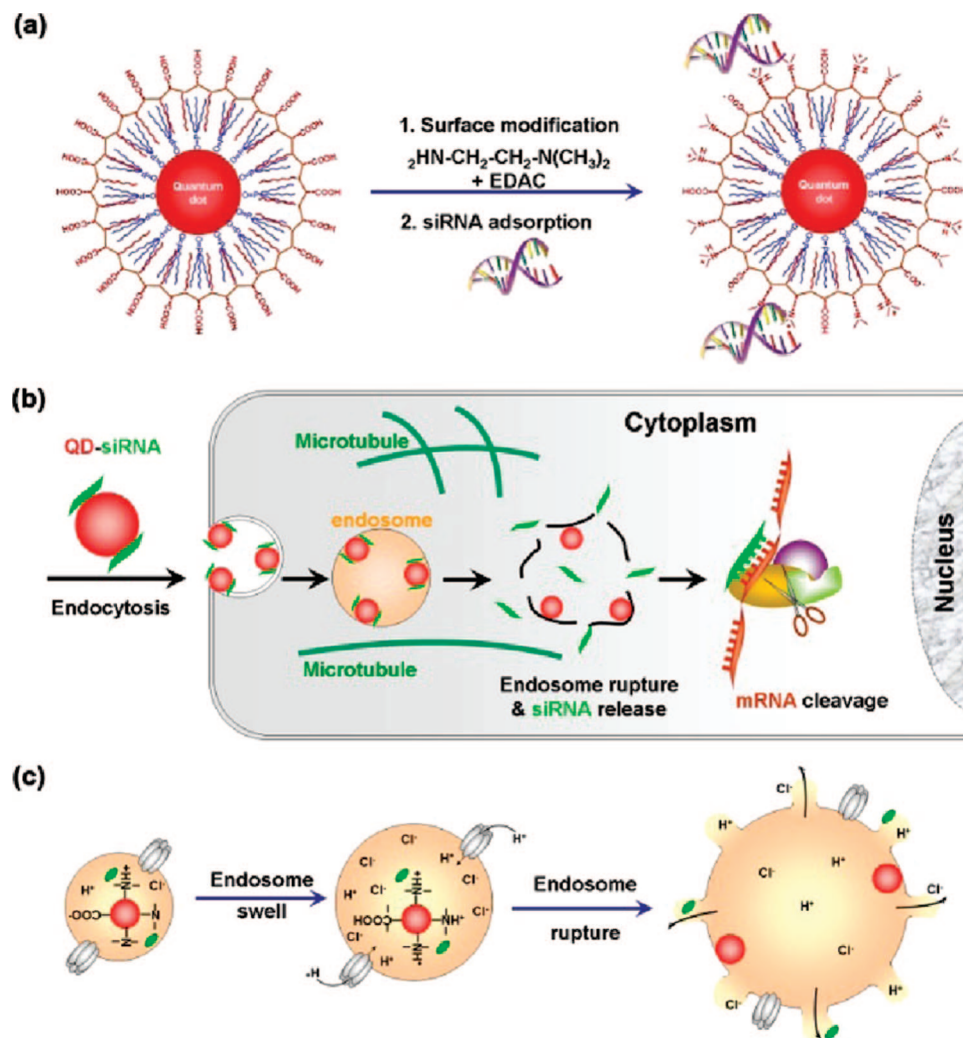
Figure 1. Rational design of proton-sponge coated quantum dots and their use as a multifunctional nanoscale carrier for siRNA delivery and intracellular imaging. (a) Chemical modification of polymer-encapsulated QDs to introduce tertiary amine groups, and adsorption of siRNA on the particle surface by electrostatic interactions. (b) Schematic diagram showing the steps of siRNA-QD in membrane binding, cellular entry, endosomal escape, capturing by RNA binding proteins, loading to RNA-induced silencing complexes (RISC), and target degradation. (c) Schematic illustration of the proton-sponge effect showing the involvement of the membrane protein ATPase (proton pump), osmotic pressure buildup, and organelle swelling and rupture. For optimized silencing efficiency and cellular toxicity, the QD surface layer is composed of 50% (molar) carboxylic acids and 50% tertiary amines. The optimal number of siRNA molecules per particle is approximately 2 (as shown in the diagram).
