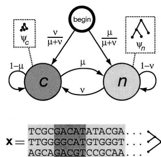
Figure 1. State-transition diagram for the phylo-HMM used by phastCons, which consists of a state for conserved regions (c) and a state for nonconserved regions (n). Each state is associated with a phylogenetic model ( \psi_c and \psi_n ); these models are identical except for a scaling parameter \rho ( 0 \leq \rho \leq 1 ), which is applied to the branch lengths of \psi_c and represents the average rate of substitution in conserved regions as a fraction of the average rate in nonconserved regions (see Methods). Two parameters, \mu and v ( 0 \leq \mu, v \leq 1 ), define all state-transition probabilities, as illustrated. The probability of visiting each state first (indicated by arcs from the node labeled “begin”) is simply set equal to the probability of that state at equilibrium (stationarity). The model can be thought of as a probabilistic machine that “generates” a multiple alignment, consisting of alternating sequences of conserved (dark gray) and nonconserved (light gray) alignment columns (see example at bottom).
