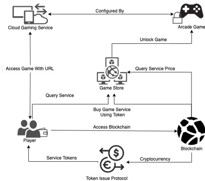
Fig. 1. System Overview of CryptoArcade
