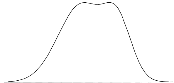
Figure 6. Mixture of two normal densities with \sigma_1 = 0.6\sigma_2 , |\mu_2 - \mu_1| = \sigma_1 + \sigma_2 , p = .288 . This density has the most pronounced dip of any mixture in which 0.6 \leq \sigma_1/\sigma_2 \leq 1 and |\mu_2 - \mu_1| \leq \sigma_1 + \sigma_2 .
