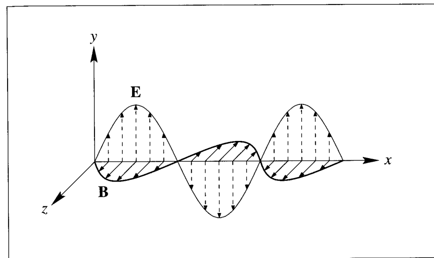
Fig. 2.2. For a given moment in time, the electric field strength \mathbf{E} and the magnetic field strength \mathbf{B} are shown along a line parallel to the direction of motion of the harmonic plane wave.
