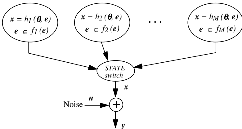
Figure 4.18 Illustration of a random process generated by a finite state system.
