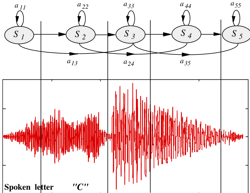
Figure 5.5 A 5-state left-right HMM speech model.
