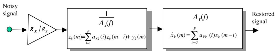
Figure 8.15 A cascade implementation of the LP squared-root Wiener filter.
