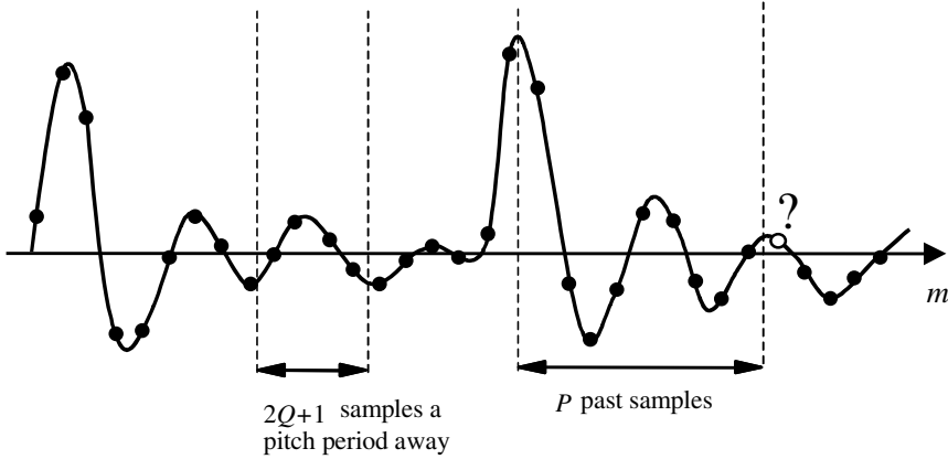
Figure 10.10 A quasiperiodic waveform. The sample marked “ ? ” is predicted using P immediate past samples and 2Q+1 samples a pitch period away.
