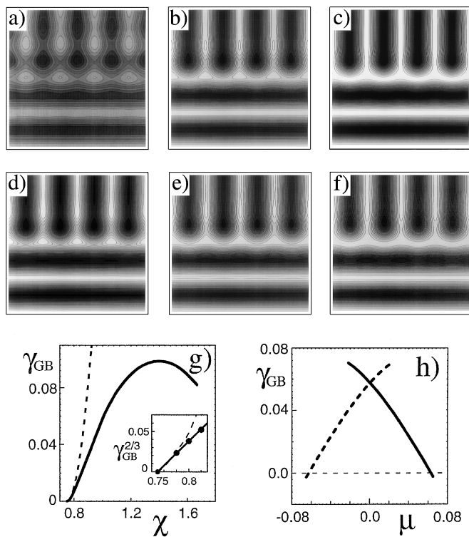
FIG. 2. Grain boundary (GB) between two perpendicular lamellar phases. (a)–(c) Contour plots of the order parameter profiles for \mu = 0 and \chi = 0.78, 1, 1.5 ; throughout the article the order parameter range [-1, 1] is represented by 20 gray scales. (d)–(f) Profiles for \chi = 1 and \mu = -0.02, 0.02, 0.06 . (g) GB interfacial energy \gamma_{GB} for \mu = 0 as a function of \chi , showing asymptotic scaling with an exponent \mu_* = 3/2 (inset). The dashed line gives the surface free energy density of one lamellar layer for comparison. (h) \gamma_{GB} for \chi = 1 as a function of \mu for two GB configurations which are degenerate at \mu = 0 , but distinct otherwise.
