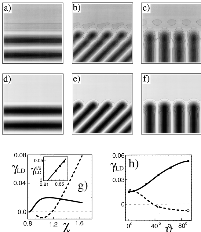
FIG. 4. Lamellar-disordered interface. (a)–(c) Profiles for \chi = 1 and different angles \vartheta = 0^\circ , 45^\circ , and 90^\circ between the lamellae and the interface. (d)–(f) Profiles for \chi = 1.5 . (g) Interfacial energy \gamma_{LD} for \vartheta = 90^\circ (dashed line) and \vartheta = 0^\circ (solid line), the latter scaling with \mu_* = 2 on approach to the metastable tricritical point (inset). (h) \gamma_{LD} as a function of the angle \vartheta for \chi = 1 (dashed line) and for \chi = 1.5 (solid line).
