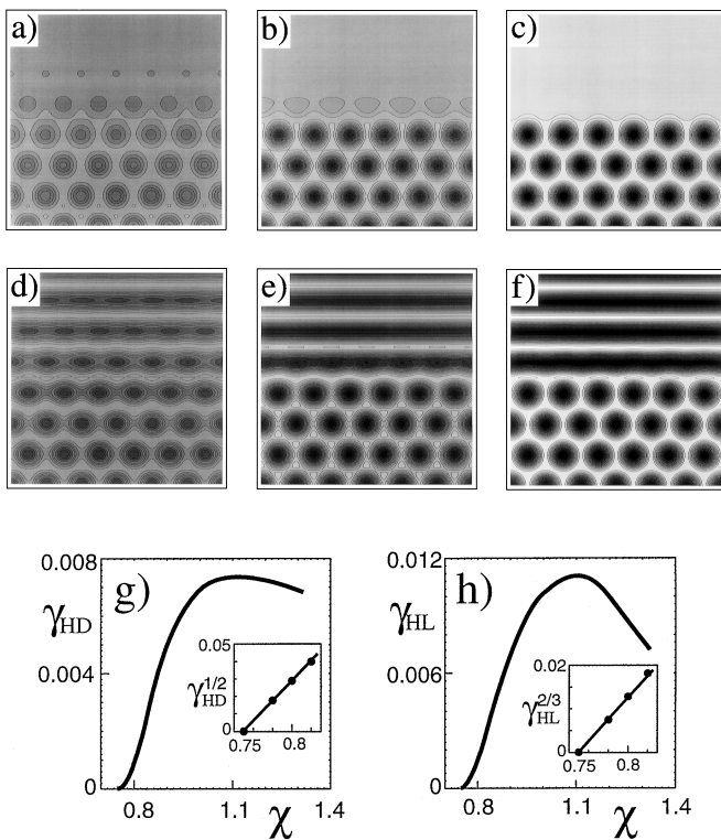
FIG. 5. (a)–(c) Hexagonal-disordered interfacial profiles for \chi = 0.78, 0.9, and 1.2 . (d)–(f) Hexagonal-lamellar profiles for \chi = 0.78, 0.9, and 1.2 . (g) Interfacial energy \gamma_{HD} along HD coexistence as a function of \chi , scaling with \mu_* = 2 (inset). (h) \gamma_{HL} as a function of \chi , scaling with \mu_* = 3/2 (inset).
