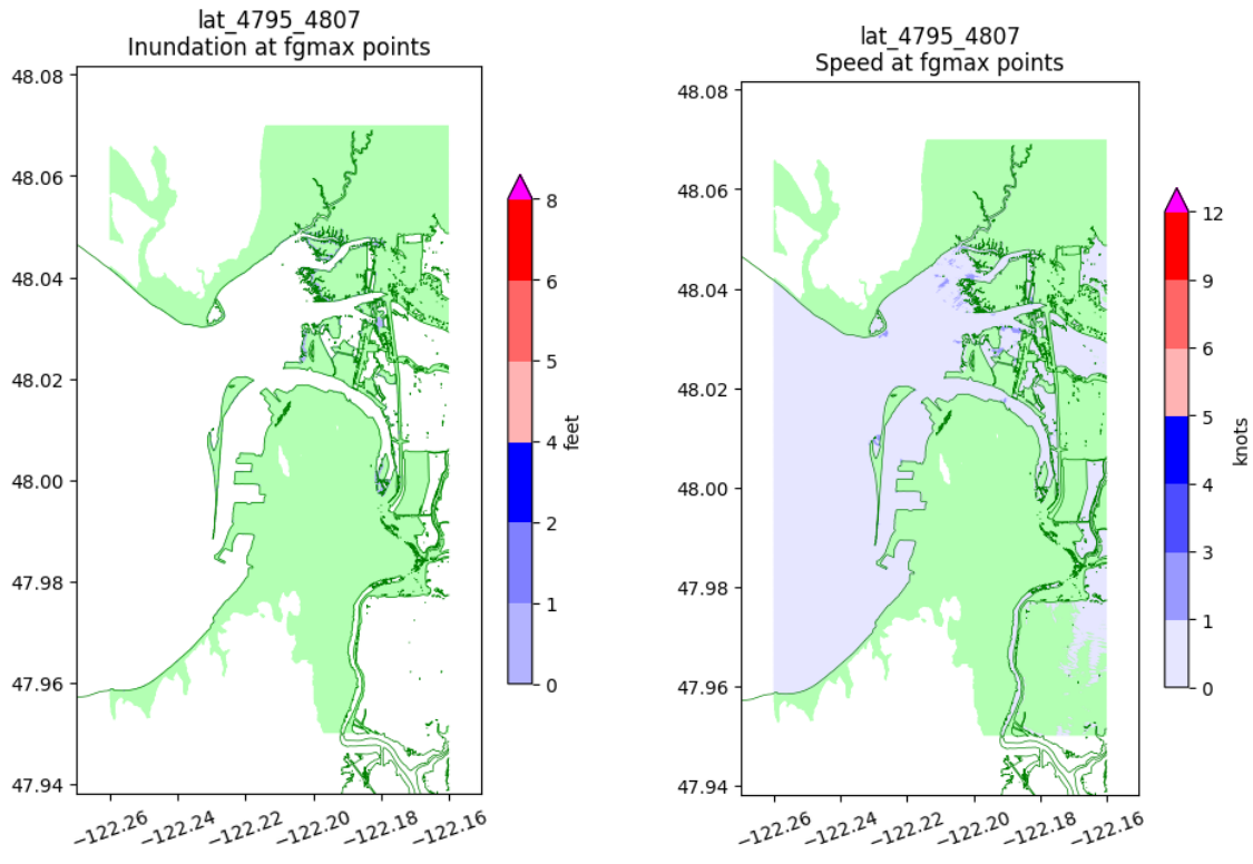
Figure 28: Maximum flow depth (left) and speed (right) calculated near Everett using our best guess at the proper SF-S model. Compare to Figure 16, which shows results with the SF-L model.
