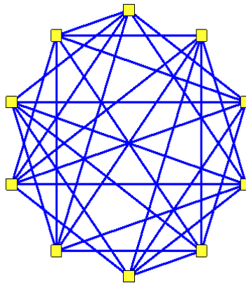
The graph G_1 10 vertices, regular of degree 6.
