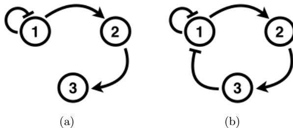
Figure 2: Two possible repairs for the GRN from Fig. 1. (a) A minimal repair (diameter=2). (b) A repair that minimizes the diameter of the graph (diameter=1).
