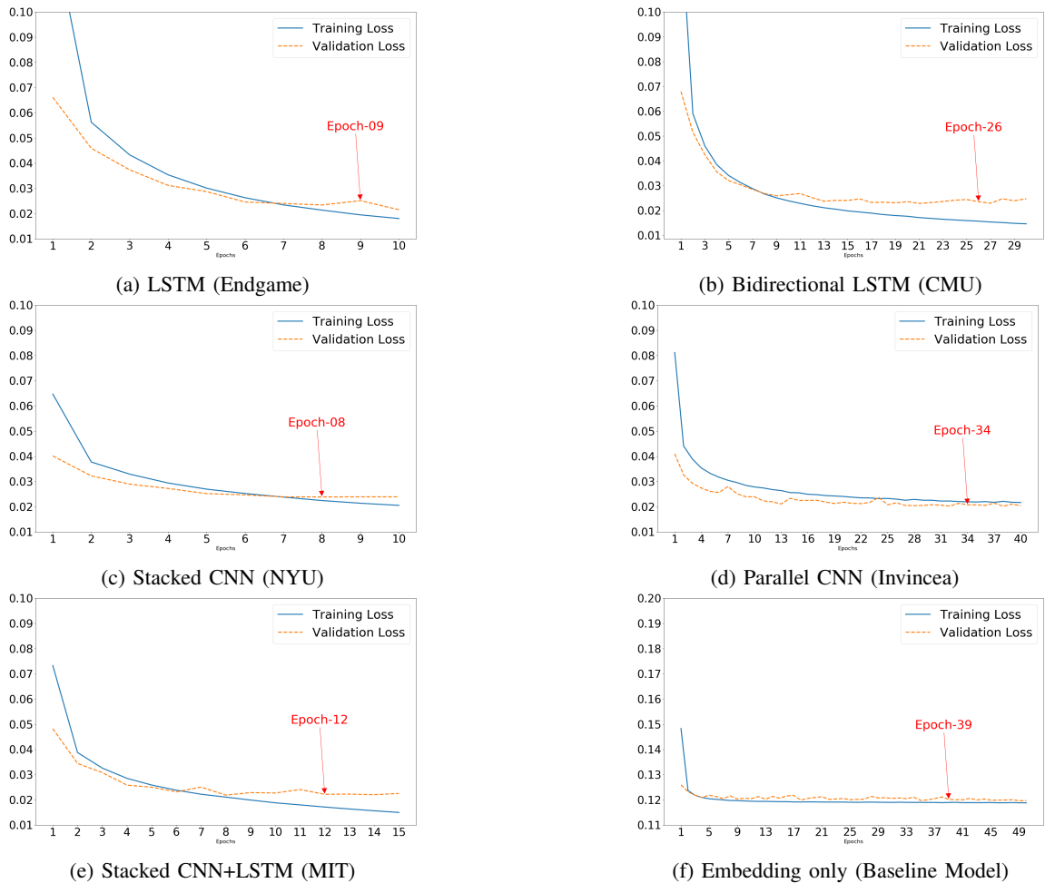
Fig. 1: Training and validation loss curves. The vertical axis in Figure (f) has a different scale than the other figures, related to the fact that the “Embedding only” baseline model has a much higher loss than the other models.
