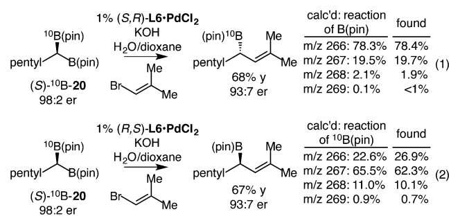
Scheme 4. Analysis of the Stereochemistry of Transmetalation in Cross-Couplings with L6-PdCl 2
