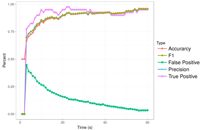
Figure 4: Time to Convergence
