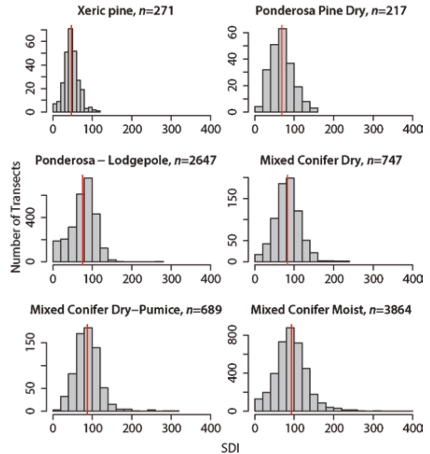
Appendix 4, Figure 1: Distribution of Stand Density Index (SDI) in historical dry forests derived from a roughly 20% sample of >200,000 acres compiled between 1914–1925 on the Klamath and Warm Springs Indian Reservations by the Bureau of Indian Affairs (BIA) (See page 94.). These BIA timber inventories include all conifers > 6" dbh on transects which were typically 20 x 2 chains (1/4 mile x 132 ft) and covered a 4-acre area. Histograms show the distribution of transect means for each habitat type. Average SDI is indicated with a red line. Boundaries for habitat types were derived from the Integrated Landscape Assessment Project potential vegetation type map (Figure 4) (ILAP 2012).
