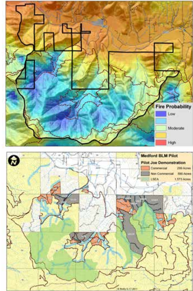
Figure 18. Top: Fire probability In Pilot Joe varies from relatively high in the valley bottom to relatively low in higher elevations. The Pilot Joe area regularly experiences both lightning strikes and human-caused ignitions; most of the fires start in the valley bottom. Bottom: Integration of forest restoration with conservation of the Northern Spotted Owl in Dry Forests of the Applegate River Drainage. Colored areas are BLM lands; white areas are private lands; blue linear features are Riparian Reserves; green areas are Late Successional Emphasis Areas (LSEAs) located around nest sites of the Northern Spotted Owl; orange areas are commercial restoration treatments that will provide economically viable timber sales; grey areas are non-commercial restoration treatments that will require investment.
