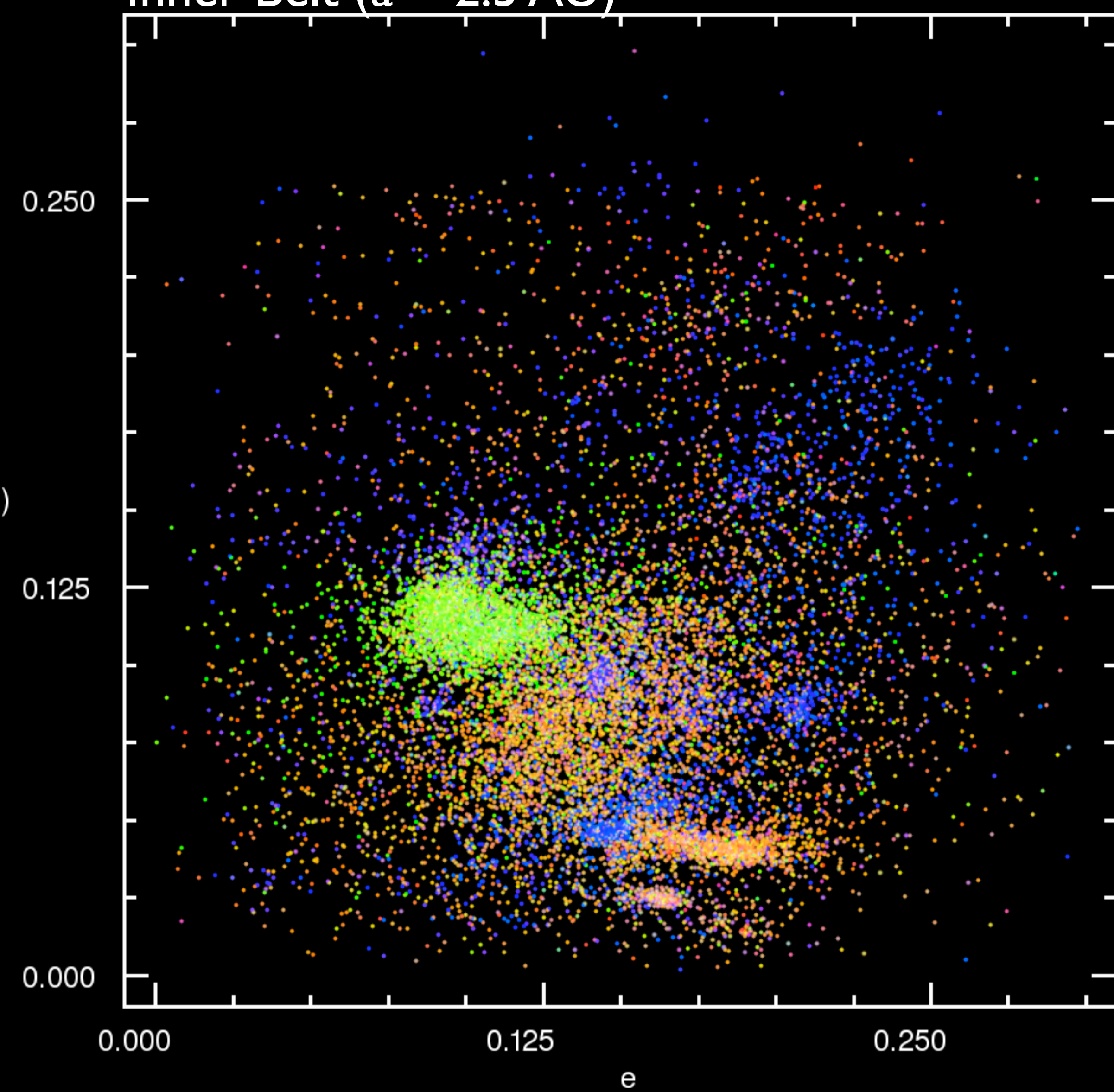
Families (Parker et al 2008)
