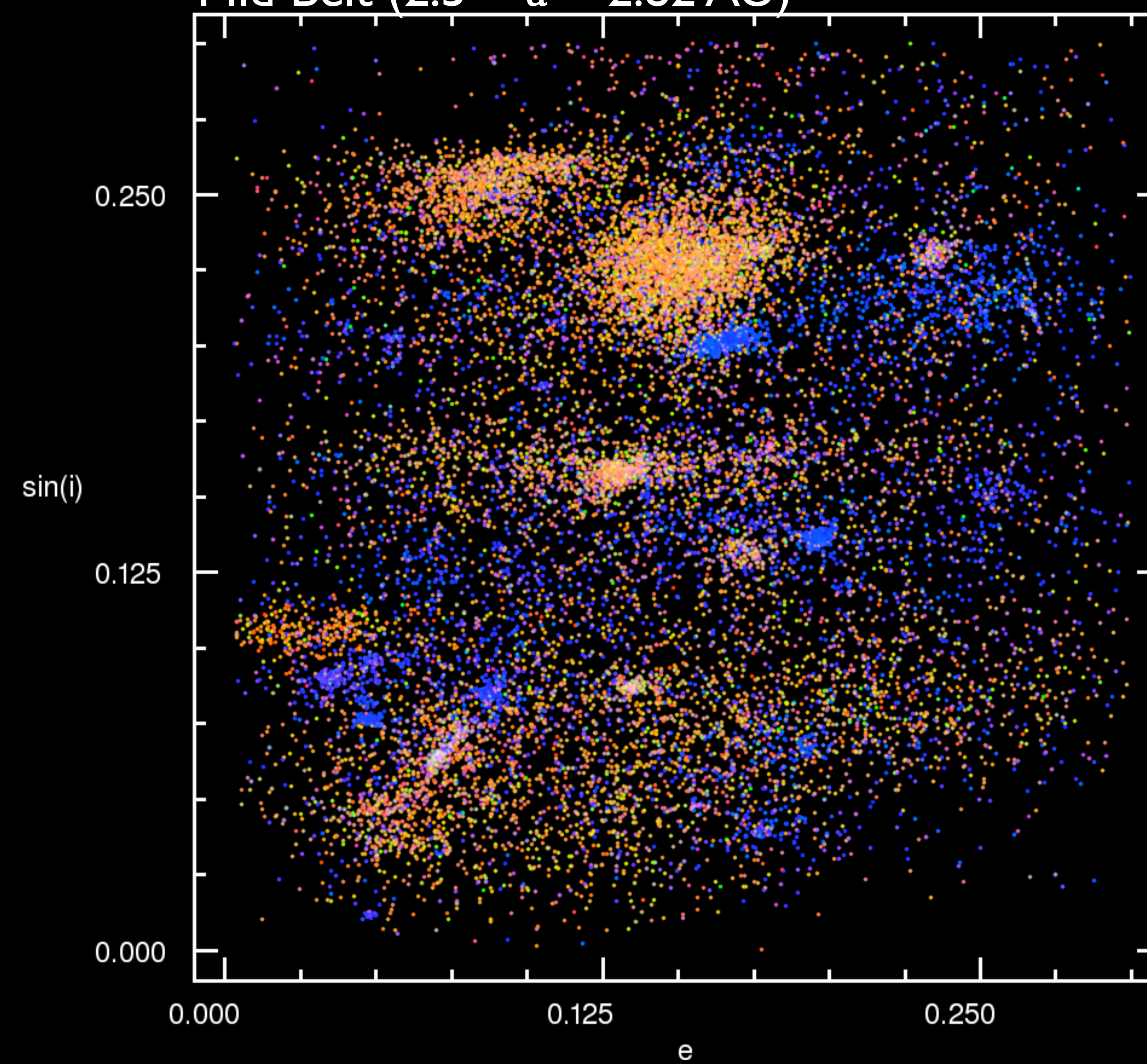
Mid Belt ( 2.5 < a < 2.82 AU)
