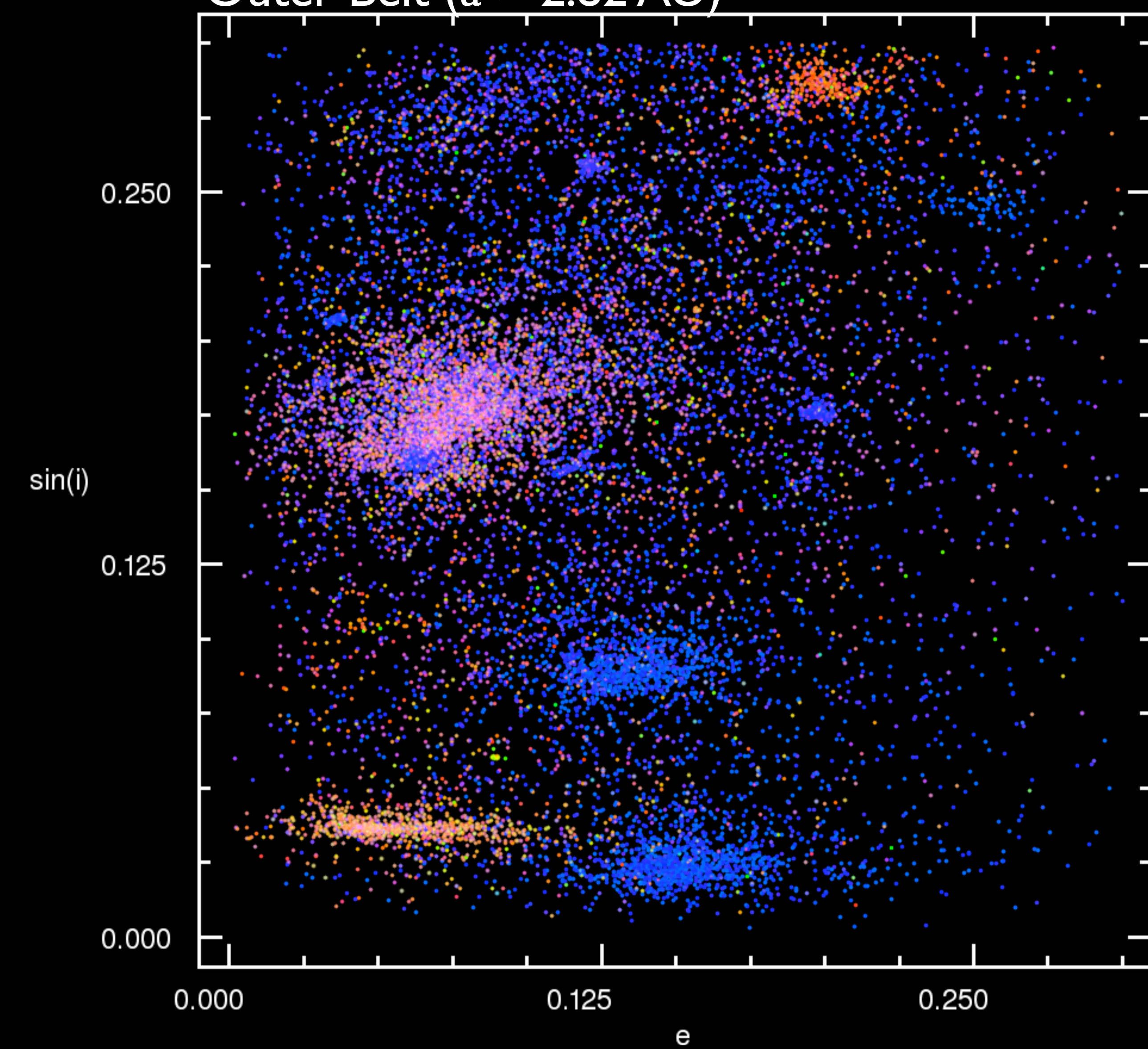
Outer Belt ( a > 2.82 AU)
