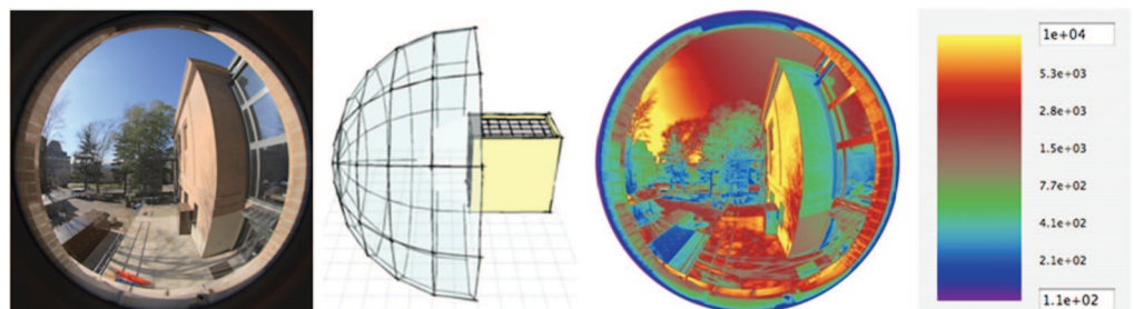
Fig. 13. Vertical fisheye image taken outside the window of the office is used as the lights source in the IBL technique to simulate the office interior.
