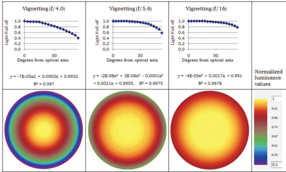
Fig. 3. Vignetting function of the fisheye lens is determined as the camera is rotated in 5° intervals away from the target, the camera response function for each aperture is determined as a polynomial fit (top row), and used to create a digital filter (bottom row) that is applied as a post process to compensate for the light fall off.
