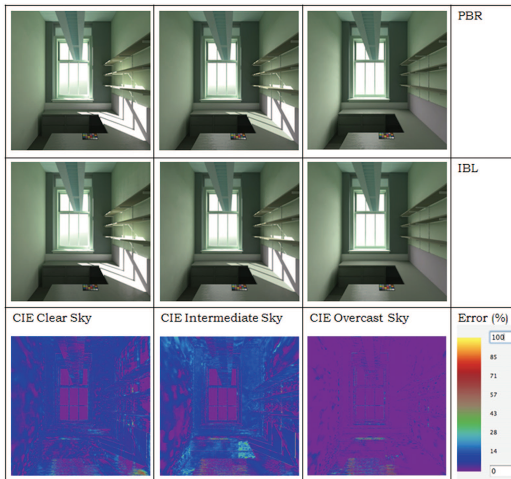
Fig. 8. Comparison of the office simulated with CIE clear, intermediate and overcast skies for March 21, 15:00: the images in the first row are generated with the mathematical model of the corresponding CIE sky (PBR), the second row images utilizes the image (IBL) of the CIE sky generated based on the mathematical model; the third row displays the error percentages when the PBR technique is compared with IBL.
