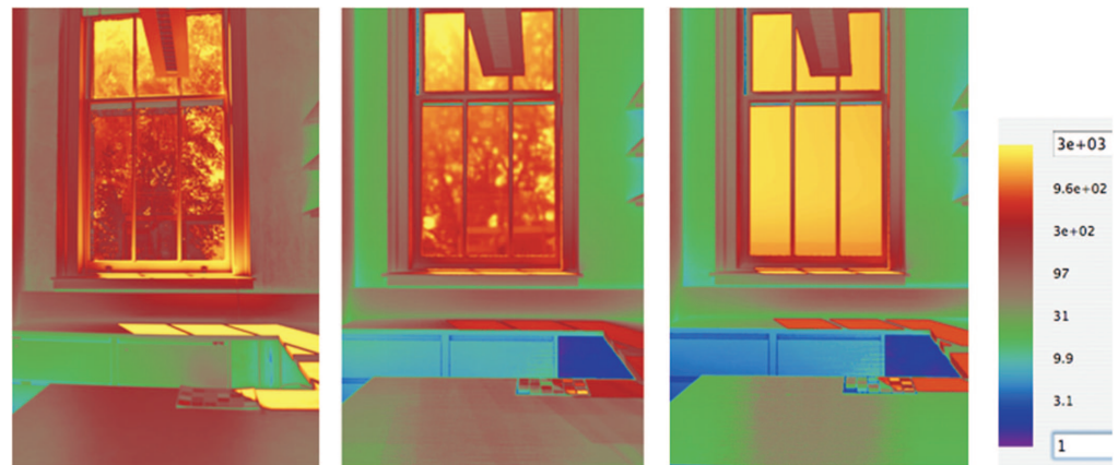
Fig. 15. Comparison of the HDR image of the sky, IBL simulation, and PBR simulation under clear sky conditions for July 29, 16:00.
