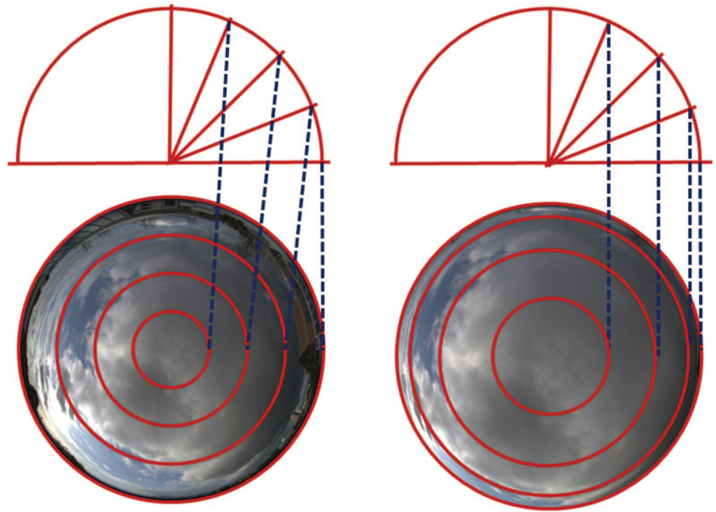
Fig. 5. Equi-distant (left) fish-eye image of the sky is transformed into hemispherical fisheye projection (right): a hemispherical fisheye image demonstrates the volume seen by the illuminance meter as measurements are taken.
