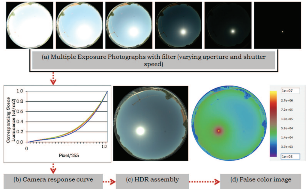
Fig. 2. Multiple exposure photographs taken with two aperture sizes (f/4 and f/16) and varying shutter speeds.
