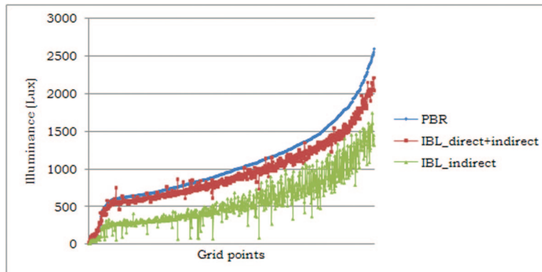
Fig. 10. Comparison of illuminance values between the PBR technique, IBL technique with indirect calculation, and IBL technique with incorporated direct and indirect calculation for June 21 14:00 under clear sky conditions.
