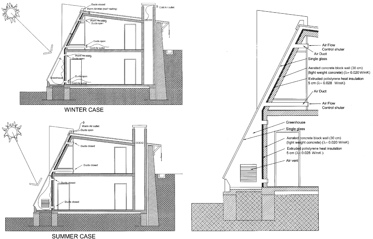
Fig. 3. Winter and summer operations of the building and detail from the isolated systems Trombe walls and greenhouse also showing the materials.
