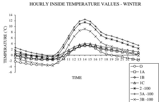
Fig. 8. Hourly values of inside temperatures of Alternatives 1A–1C, and 100% ratio of fenestration to facade area (window/total) of Alternatives 2, 3A, and 3B, 2–100, 3A–100, and 3B–100.
