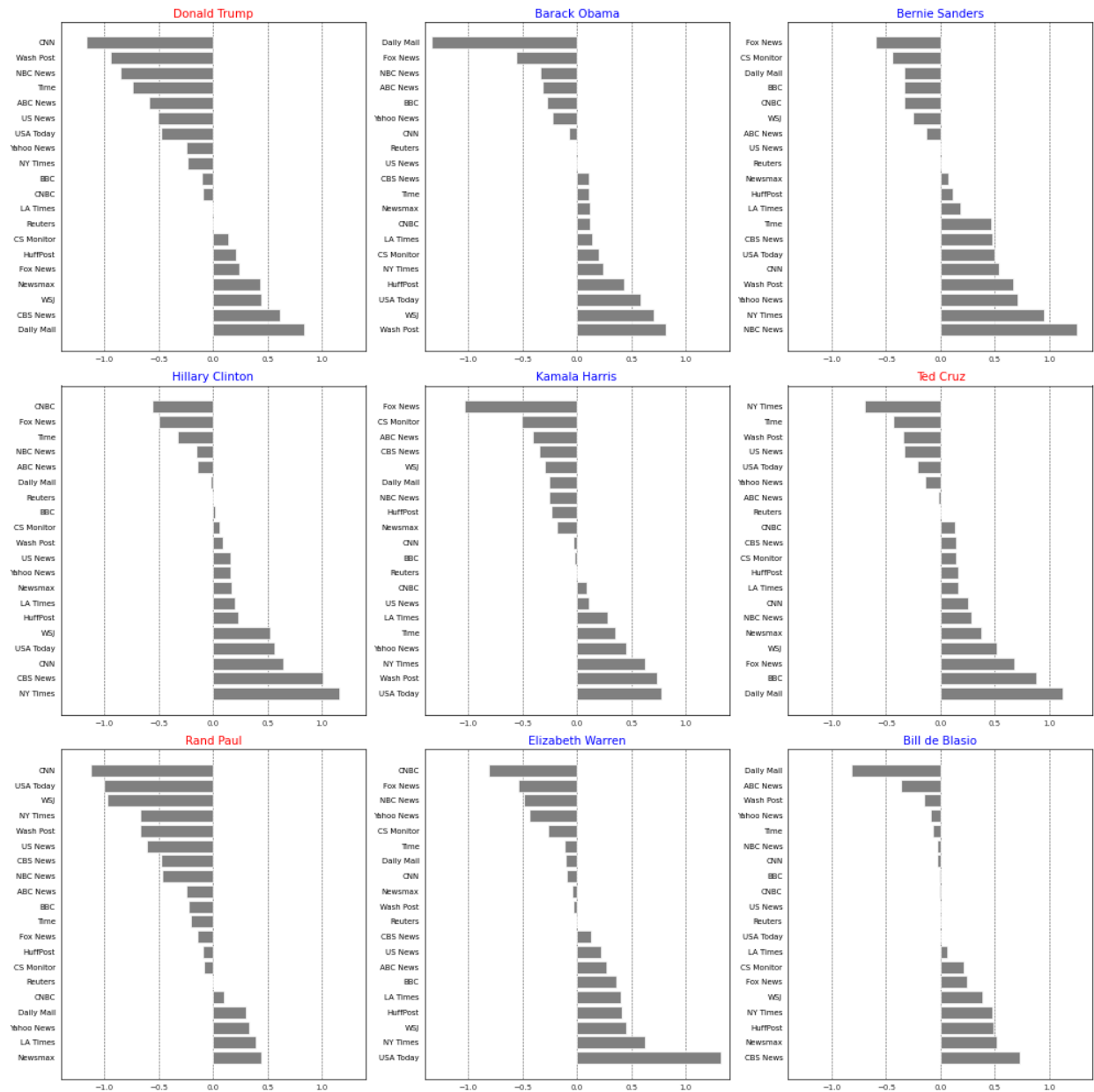
Figure A.13: Bar plot showcasing the polarization across various Politicians, segmented by different News Outlets, Part I
