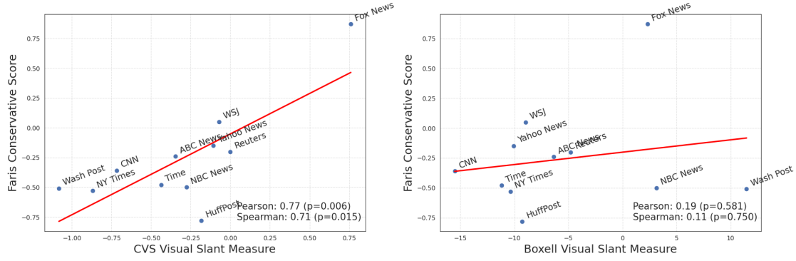
Figure A.10: Comparison of visual slant from our PMCIG method (left) and Boxell (2021) approach (right) against the conservative score from Faris et al. (2017).
