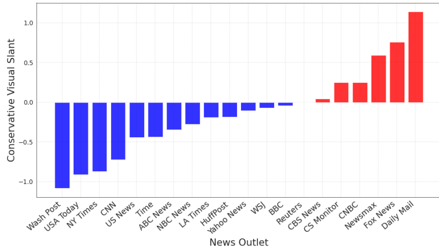
Figure 12: Conservative Visual Slant (CVS) of news outlets.
