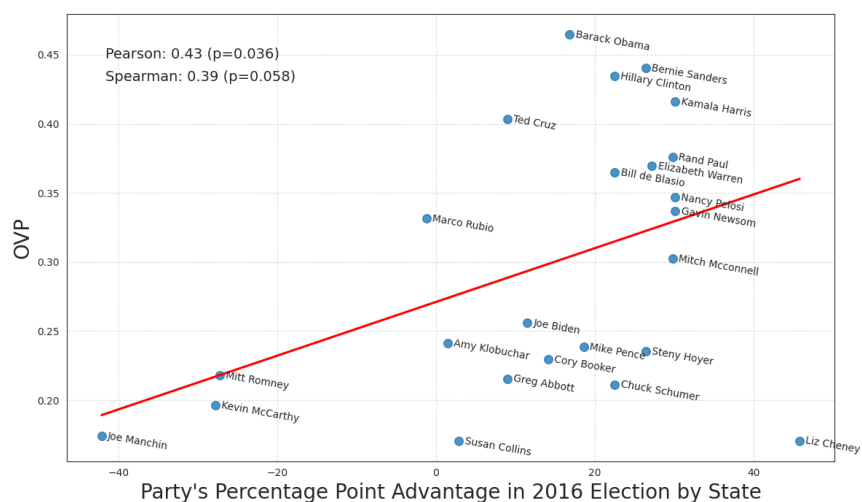
Figure 16: Relationship between a politician's Overall Visual Polarization (OVP) and their ideological alignment with their constituency.
