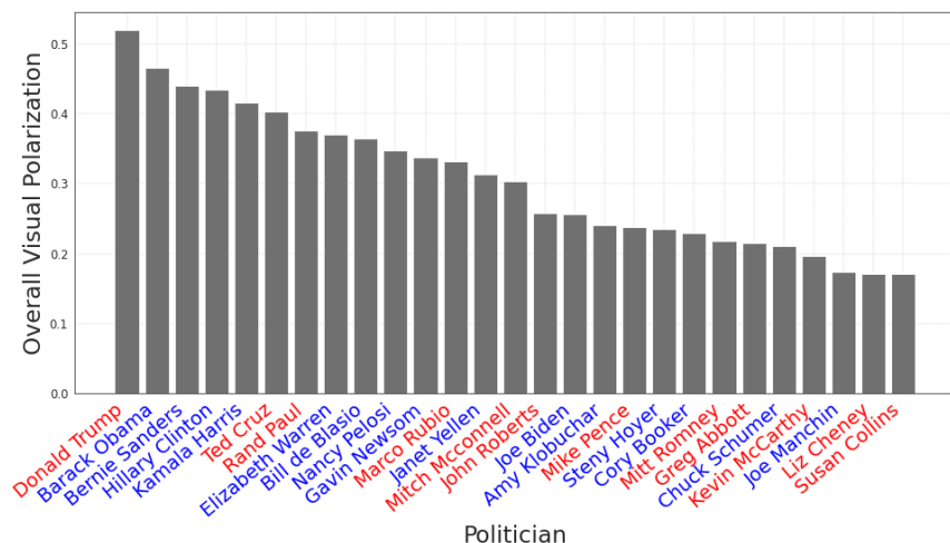
Figure 15: Overall Visual Polarization (OVP) of politicians across all news outlets, ranked from most to least polarized.
