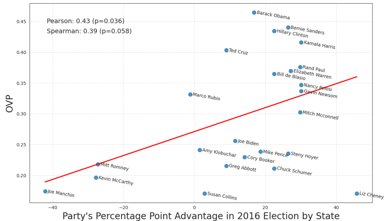
Figure A.16: Relationship between state partisanship and politician's Overall Visual Polarization
