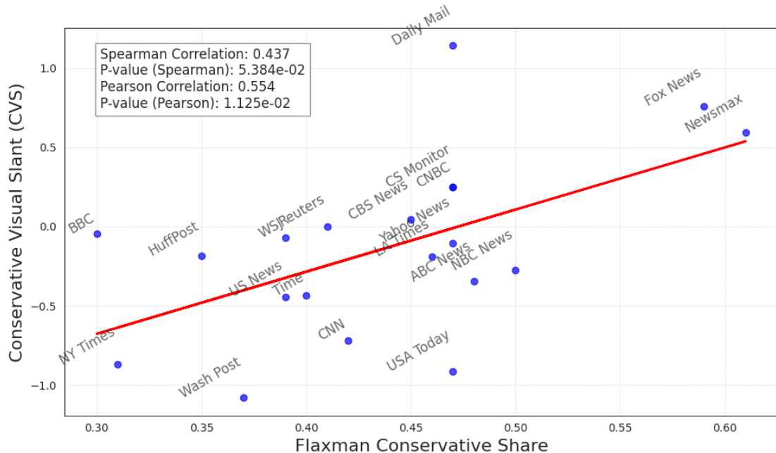
Figure A.9: Correlation between CVS and the conservative share score of news outlets. (Based on Flaxman et al. (2016) Conservative Score)
