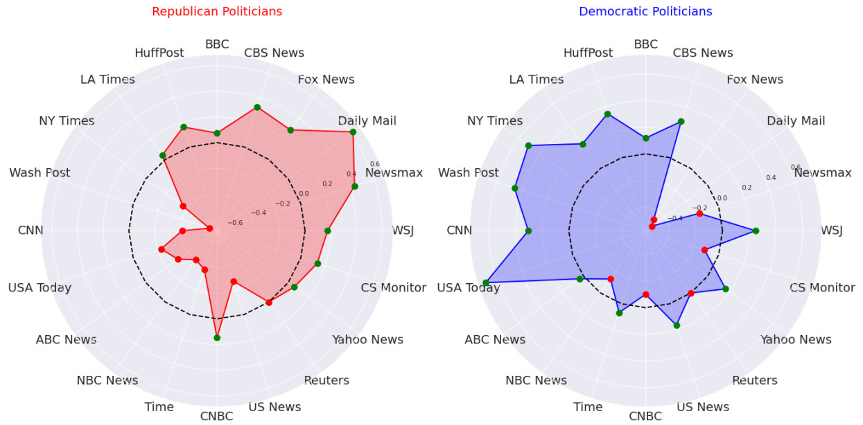
Figure A.5: Radar plots showing the mean polarization measurement for Republican and Democratic politicians across various news outlets. Reuters polarization is zero since it serves as the baseline.
