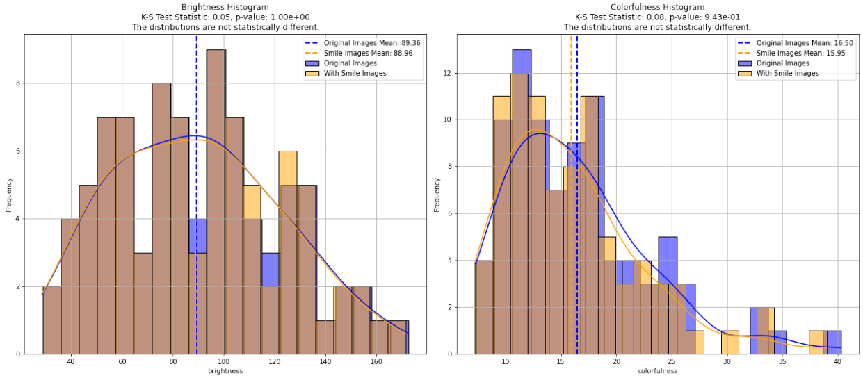
Figure A.4: Histograms of brightness and colorfulness for original and smiley images.
