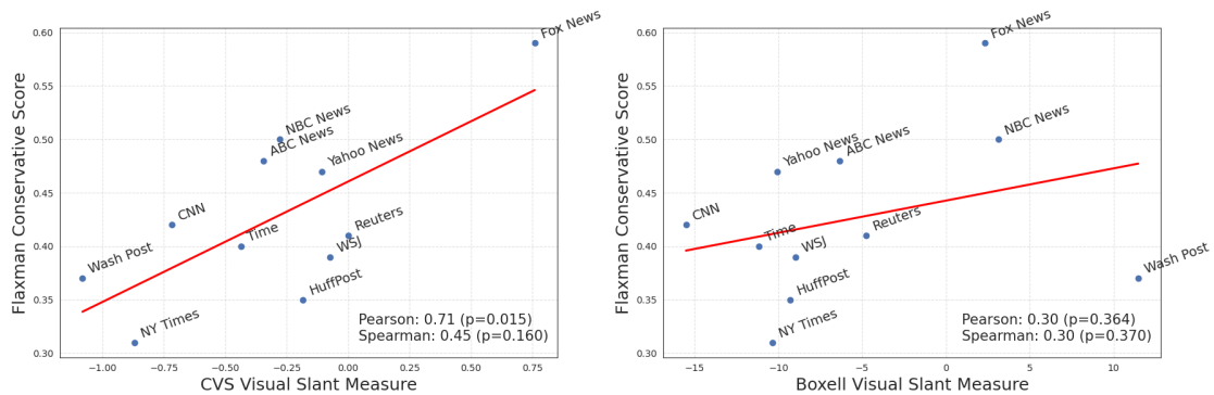
Figure A.12: Comparison of visual slant from our PMCIG method (left) and Boxell (2021) approach (right) against the conservative score from Flaxman et al. (2016).
