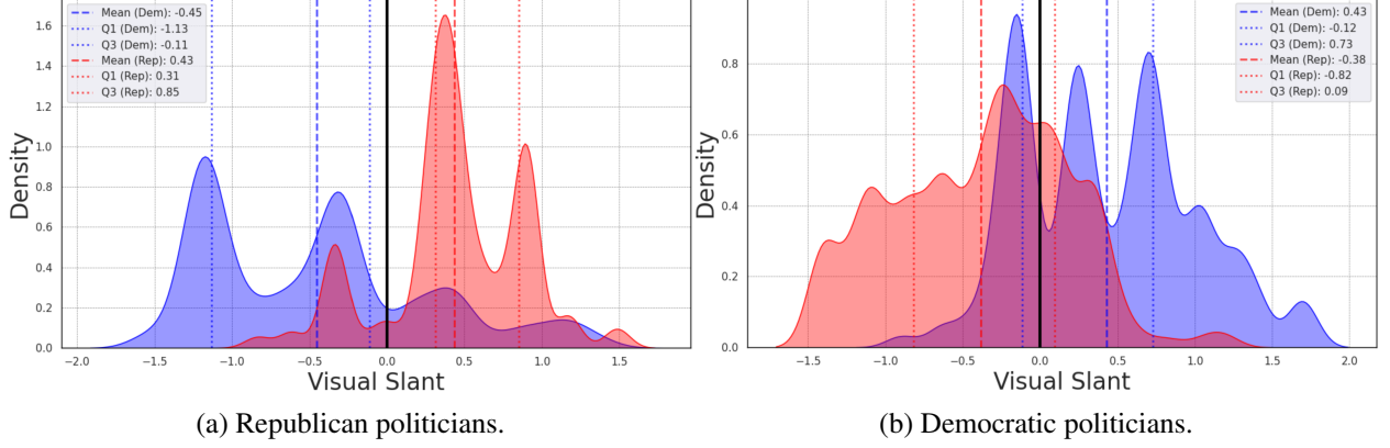
Figure 10: Histograms of visual slant for Democratic and Republican Politicians in Democratic- and Republican-leaning News Outlets.
