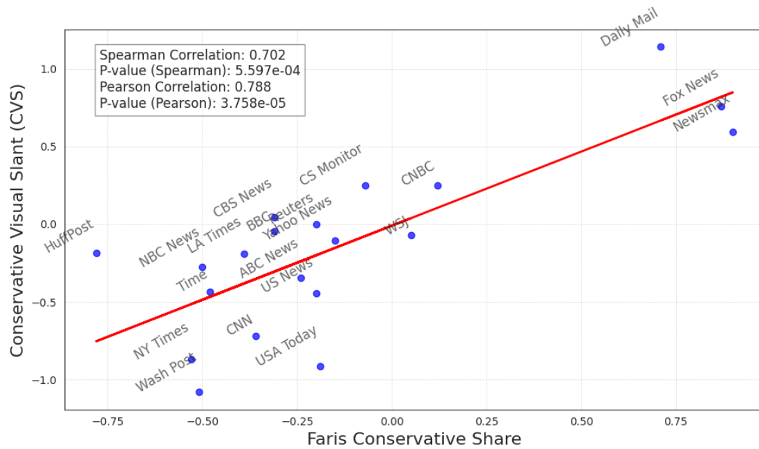
Figure A.7: Correlation between CVS and the conservative share score of news outlets (based on Faris et al. (2017) 's Conservative Score).
