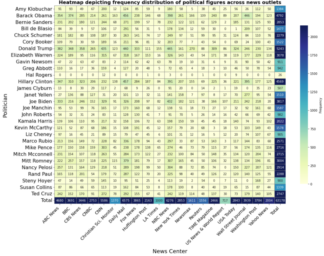
Figure A.3: Frequency distribution of politicians across outlets.
