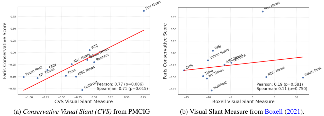
Figure 13: Comparison of CVS and visual slant measure by Boxell (2021) against Conservative Share Score from Faris et al. (2017) .
