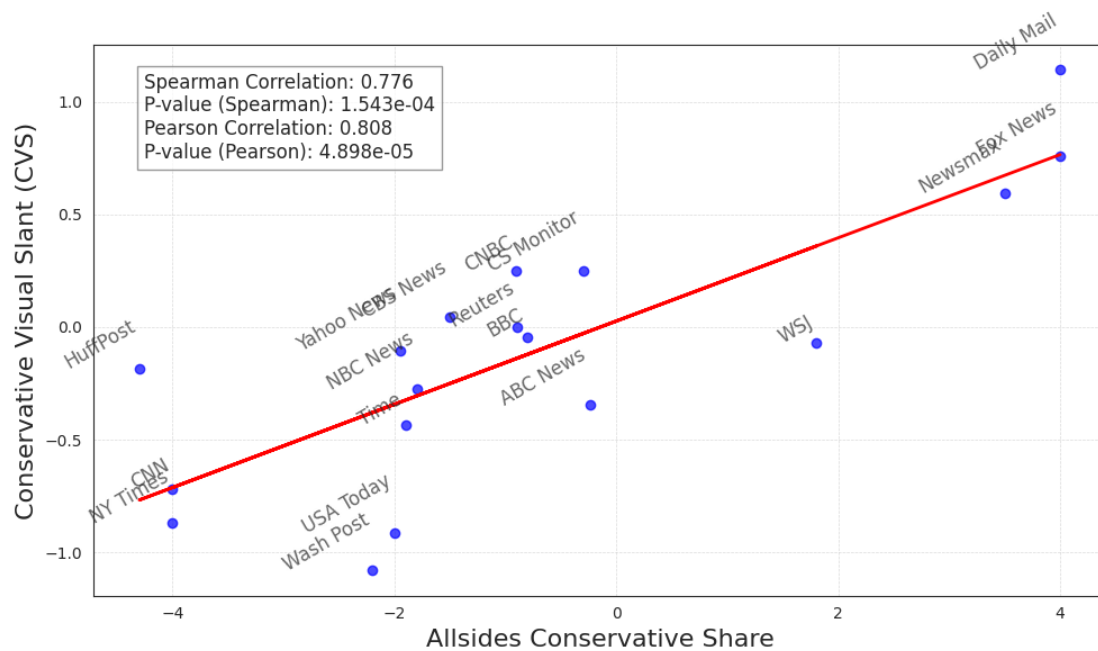
Figure A.8: Correlation between CVS and the conservative share score of news outlets (based on AllSides (2024) 's Conservative Score).
