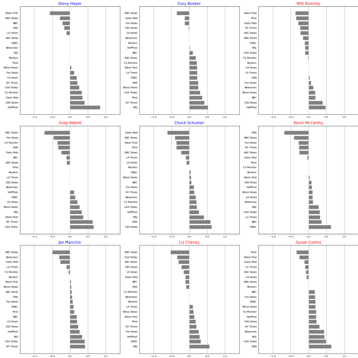
Figure A.15: Bar plot showcasing the polarization across various Politicians, segmented by different News Outlets, Part III
