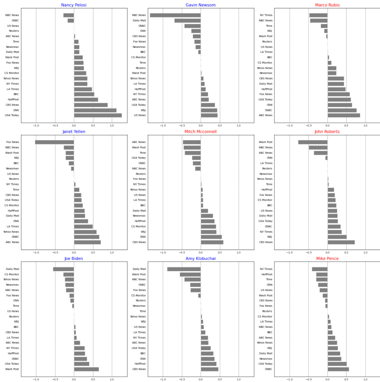
Figure A.14: Bar plot showcasing the polarization across various Politicians, segmented by different News Outlets, Part II
