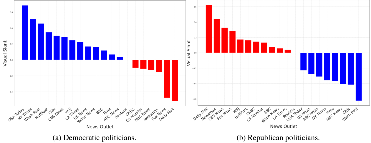
Figure 11: Overall visual slant measures for Democratic and Republican politicians by news outlet.
