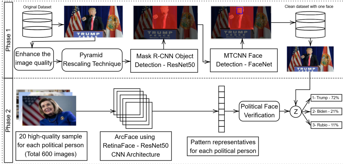
Figure A.2: Two-phase computer vision framework for political person verification.
