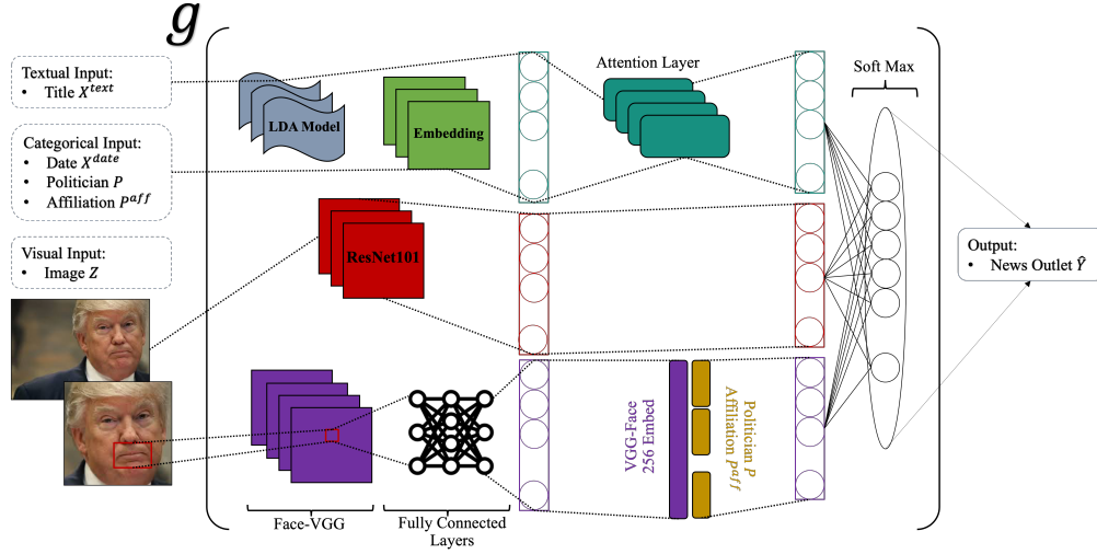
Figure 6: The multi-modal deep learning model for the news outlet prediction task
