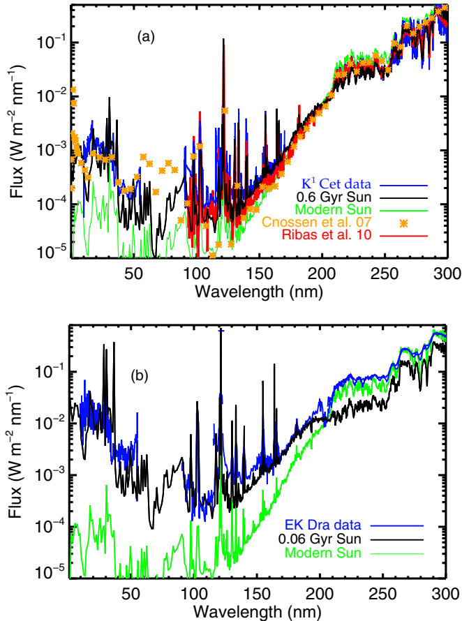
Figure 9. (a) Comparison of model predictions to available data for \kappa^1 Cet. Data, shown as a (blue) line, are from EUVE (10–70 nm), FUSE (90–119 nm), and HST -STIS (120–300 nm). The high-resolution spectral flux (at top of Earth’s atmosphere) for the Sun at 0.6 Gyr from this study is shown as a thick black solid line, with the modern solar flux shown for comparison as a thin green solid line. The Cnossen et al. (2007) modeled flux at 1 AU from \kappa^1 Cet is shown as (orange) “*” symbols (Cnossen et al. 2007). (b) EK Dra data are shown as (blue) “+” symbols and are taken from EUVE (10–70 nm), FUSE (90–119 nm), and Segura et al. (2007; 115–300 nm). The Sun at 0.1 Gyr as predicted by this study is shown as a thick gray solid line, with the modern Sun shown for comparison as a thin gray solid line.
