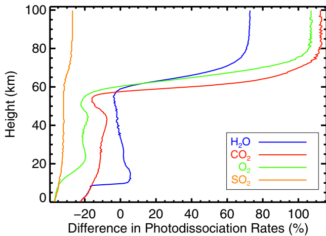
Figure 10. Change [(\text{Archean rates} - \text{Modern rates})/\text{Modern rates}] in photolysis rate constants ( \text{s}^{-1} ) computed in two one-dimensional Archean photochemical model runs. The model runs differed only in the top of the atmosphere solar flux, with one using the modern solar flux and the other using the solar flux from 3 billion years ago as predicted by our model.
