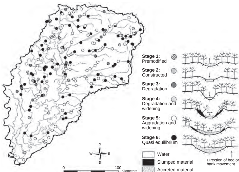
Figure 5.1 Using reconnaissance survey and rapid assessment protocols and to characterize sites in the Yazoo River catchment, Mississippi, according to their stage in river bed and bank erosion (see legend) following the passage of multiple knickpoints (adapted from Simon et al., 2007b)
