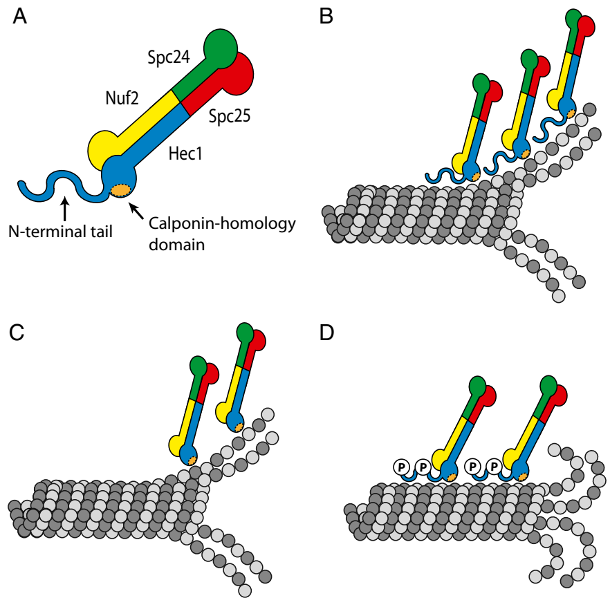
Fig. 1. (A) Human Ndc80 complex: Hec1 (blue) contains a calponin-homology domain (orange) and an unstructured N-terminal tail, Nuf2 (yellow), Spc24 (green), and Spc25 (red). (B) WT Ndc80 complex slows microtubule disassembly, promotes rescue, and stabilizes straighter protofilaments. (C) Mutated Ndc80 complex with a deleted N-terminal Hec1 tail has a lower affinity for microtubules but still slows disassembly, promotes rescue, and stabilizes protofilaments. (D) Alternative mutant form of the Ndc80 complex with phosphomimetic mutations on the Hec1 tail has a lower affinity for microtubules and is still able to slow disassembly but cannot promote rescue or stabilize straighter protofilaments. P represents the residues in the N-terminal tail mutated to mimic phosphorylation by Aurora B kinase.
