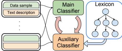
Figure 1: EZLearn architecture: an auxiliary text classifier is introduced to bootstrap from the lexicon (often available from an ontology) and co-teach the main classifier until convergence.
