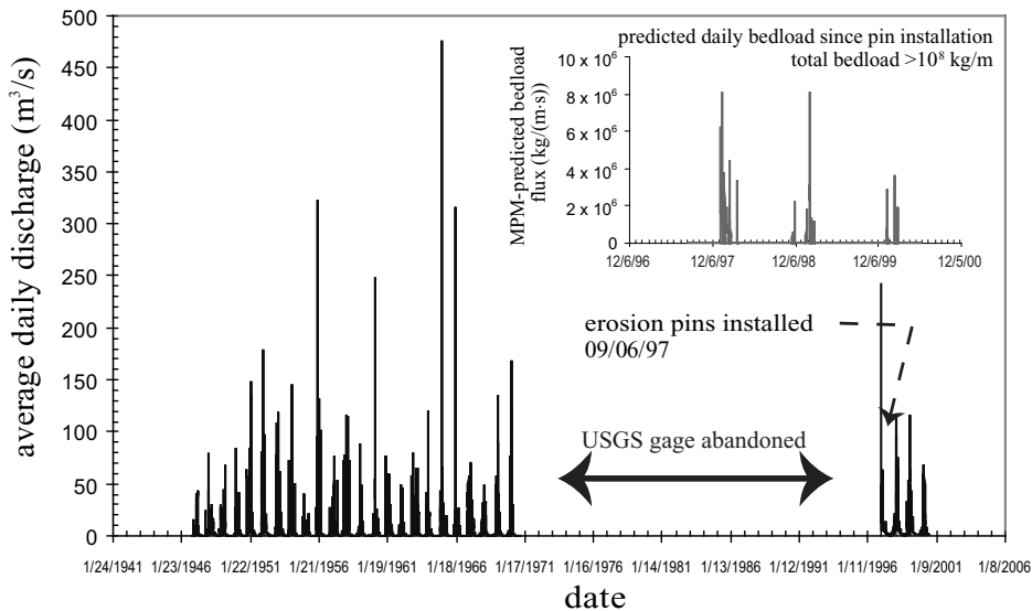
Figure 6. Average daily discharge for S.F. Eel at Branscomb gage (#11475500). Values from 1997 to 2000 are from a stage recorder operated by U.C. Angelo Reserve staff. Inset shows an illustrative calculation of bed-load transport capacity past the erosion-pin site for the period of stage record; the calculation used the Meyer-Peter and Mueller (MPM) bed-load equation as found in Julien (1998: equation 9.3a). Excess shear stress calculated by using stage data with \tau^*_c equal to 0.047 and grain-size and slope data in Table 1. These values are two orders of magnitude larger than regional values from sediment-yield estimates of bed load, consistent with excess transport capacity at this bedrock reach.
