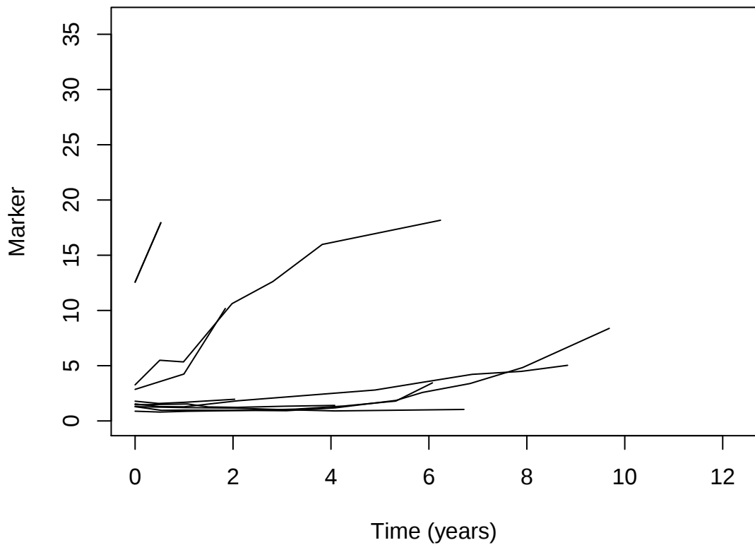
BLUP predictions
