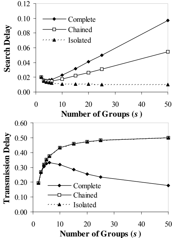
Fig. 11. The impacts of number of groups on expected search and transmission delays.
