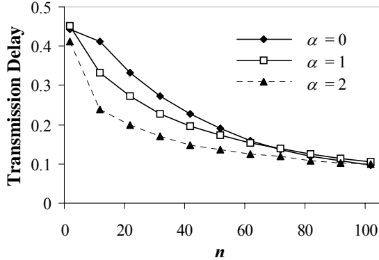
Fig. 5. Effect of \alpha on transmission delay T(n) .
