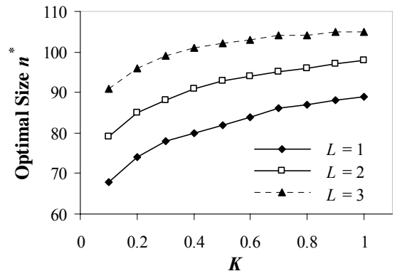
Fig. 7. Optimal size versus K and L .
