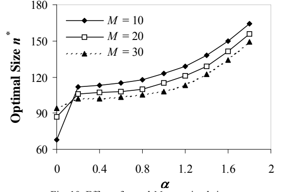
Fig. 10. Effect of \alpha and M on optimal size.
