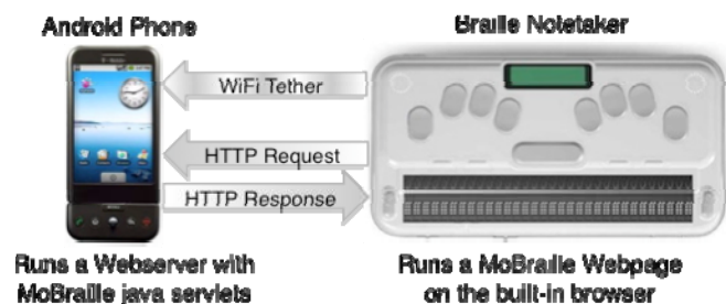
Figure 2. With MoBraille, a webpage loaded on a Wi-Fi-enabled Braille display sends HTTP requests to an Android phone and receives HTTP responses.
