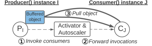
Figure 4: Zipline architecture overview.
