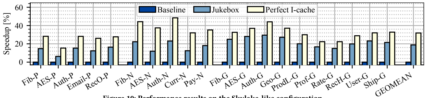
Figure 10: Performance results on the Skylake-like configuration.
