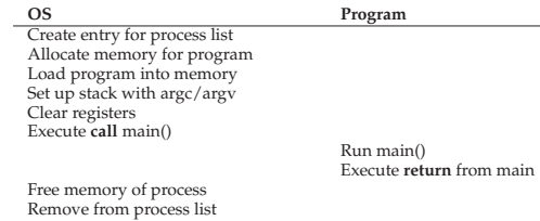
Figure 6.1: Direct Execution Protocol (Without Limits)
