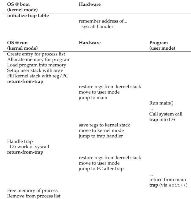
Figure 6.2: Limited Direct Execution Protocol
