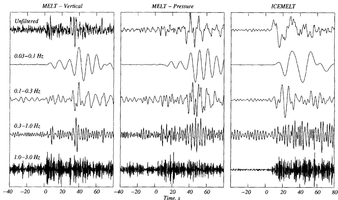
Figure 2. Examples of P waves recorded during the MELT and ICEMELT experiments. The left hand panel shows the vertical channel at MELT site 5 for an earthquake that occurred south of the Fiji Islands at 00:30 GMT on April 16, 1996 ( \Delta = 61^\circ , M = 7.1 , and Z = 111 km). The center panel shows the pressure record at a nearby site for the same earthquake. The right hand panel shows the vertical channel at ICEMELT station NYD for an earthquake near the Andreanof Islands at 15:24 GMT on June 10, 1996 ( \Delta = 63^\circ , M_s = 7.1 , Z = 26 km). Each panel shows the unfiltered record and four traces that have been filtered into the pass bands of 0.03–0.1 Hz, 0.1–0.3 Hz, 0.3–1 Hz, and 1–3 Hz. The instrument response has been deconvolved from each filtered trace and a fourth order minimum phase bandpass butterworth filter applied. The traces are plotted with equal maximum amplitude.
