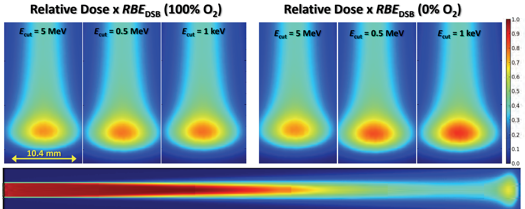
Figure 5. Effects of proton cutoff energy and oxygen level on the shape of a 163 MeV pencil (5.2 mm spot size) simulated in MCNP. Doses in all panels are normalized to the maximum physical dose for the simulation with a 1 keV proton cutoff energy and displayed using a linear color-gradient scheme. A lattice tally in MCNP was used to tally the 2D (and 3D) dose and RBE \times dose distributions. Top Panels: RBE_{DSB} \times relative dose for well oxygenated and anoxic cells. Bottom Panel: relative absorbed dose as a function of depth into water. Bragg peak occurs at a depth of \sim 185 mm (see also Figure 4 ).
