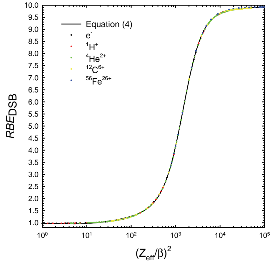
Figure 1. Estimates of RBE_{\text{DSB}} for selected ions relative to ^{60}\text{Co} \gamma -rays from the empirical fits (Eqs. 3 and 4) to estimates from MCDS simulations. Left Panel: cells irradiated under normoxic conditions ( 8.32 \text{ DSB Gy}^{-1} \text{ Gbp}^{-1} for ^{60}\text{Co} ). Right Panel: cells irradiated under anoxic conditions ( 2.86 \text{ DSB Gy}^{-1} \text{ Gbp}^{-1} for ^{60}\text{Co} ).
