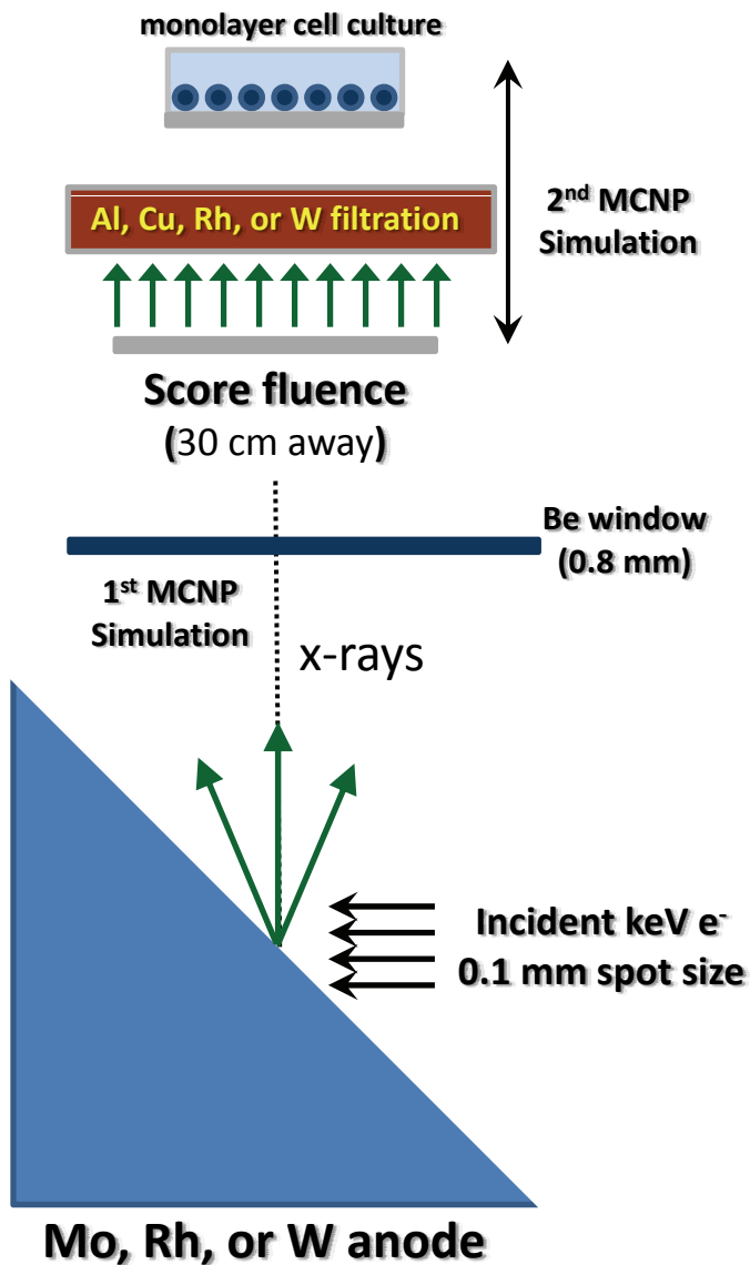
Figure 3. Left Panel: Model for an idealized (generic) x-ray machine with optional filtration. In the first stage of the MCNP simulation, electrons and photon are tracked down to a cutoff energy of 1 keV. A 1 keV electron and photon cutoff energy is also used in the Cu filter in the 2 nd stage of the MCNP simulation. In the cell culture dish, cell layer and culture medium, electrons and photons are transported down to a cutoff energy of 100 eV. Right Panel: x-ray energy spectrum from the MCNP simulation of monoenergetic 200 and 250 keV electrons incident on the W target with 1.5 and 1.3 mm of Cu filtration respectively.
