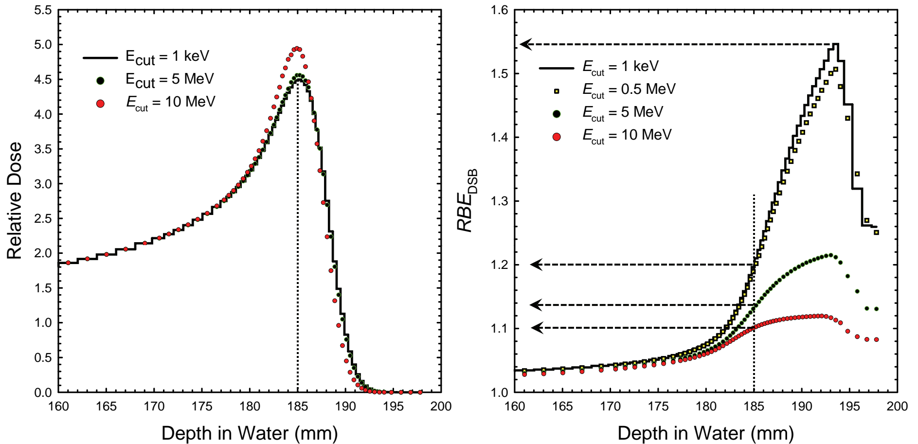
Figure 4. Effects of proton cutoff energy ( E_{cut} ) on MCNP simulations of a 163 MeV proton pencil beam incident on a 40 \times 40 \times 40 cm 3 water phantom. Bragg peak occurs at a depth of 185 mm ( vertical dashed lines ). Left Panel: absorbed dose normalized to the absorbed dose at a 2 cm depth ( not shown ). Right Panel: dose-averaged RBE_{DSB} . RBE_{DSB} value at the Bragg peak (depth = 185 mm) increases from about 1.1 ( E_{cut} = 10 MeV) to 1.2 ( E_{cut} \leq 0.5 MeV). Beyond the Bragg peak, RBE_{DSB} reaches a peak value \leq 1.55 ( E_{cut} = 1 keV).
