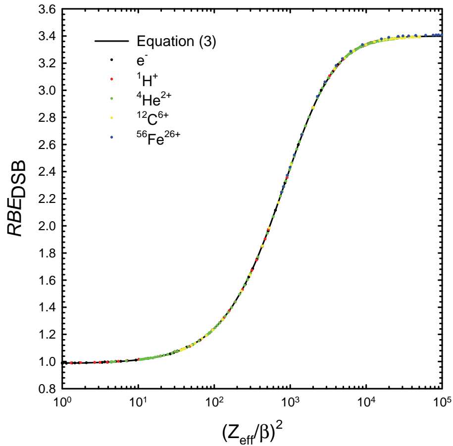
Figure 1. Estimates of RBE_{\text{DSB}} for selected ions relative to ^{60}\text{Co} \gamma -rays from the empirical fits (Eqs. 3 and 4) to estimates from MCDS simulations. Left Panel: cells irradiated under normoxic conditions ( 8.32 \text{ DSB Gy}^{-1} \text{ Gbp}^{-1} for ^{60}\text{Co} ). Right Panel: cells irradiated under anoxic conditions ( 2.86 \text{ DSB Gy}^{-1} \text{ Gbp}^{-1} for ^{60}\text{Co} ).
