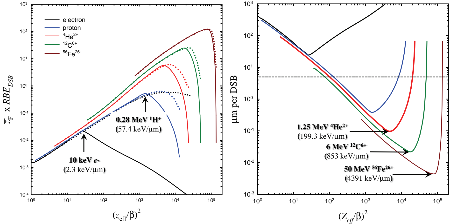
Figure 2. Left Panel: Per track estimate of the number of DSB formed by selected ions relative to {}^{60}\text{Co} \gamma -rays. Solid lines: Estimates of the frequency-mean specific energy corrected for CSDA range and changes in stopping power as particles pass through a cell nucleus 5 \mu\text{m} in diameter (MCDS simulation). Dotted lines: frequency-mean specific energy estimated using \text{LET}/\rho d^2 (LET for water from the MCDS); particle type corresponds to solid line with same color. Right Panel: average distance between DSB formed in the nucleus of a diploid human cell (6 Gbp of DNA) by a single charged particle. Horizontal dashed line indicates the diameter of the nucleus ( 5 \mu\text{m} ). Colors and line styles indicate same particle type as left panel.
