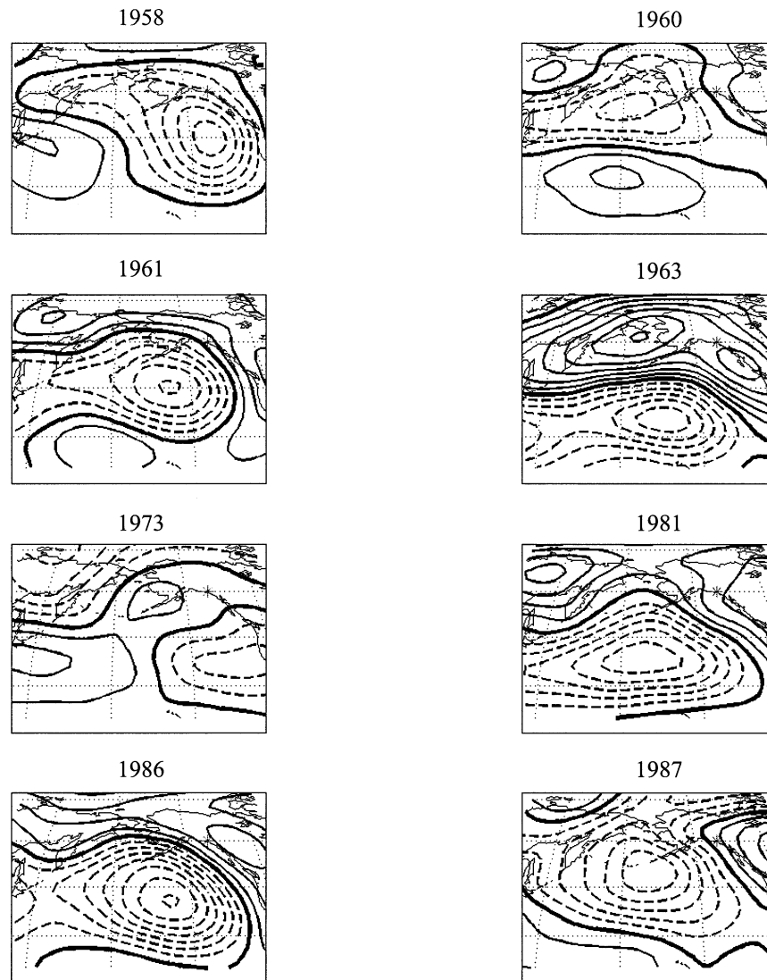
FIG. 7. The 500-hPa geopotential height anomalies for each of the anomalously high accumulation years. The contour interval is 20 m. The zero contour is bold, and the negative contours are dashed. Note that 1963 and 1973 are the most different.
