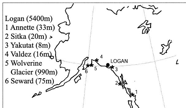
FIG. 2. Map of Alaska and part of the Yukon showing the locations and elevations of the Mt. Logan ice core (dot) and precipitation stations (stars).
