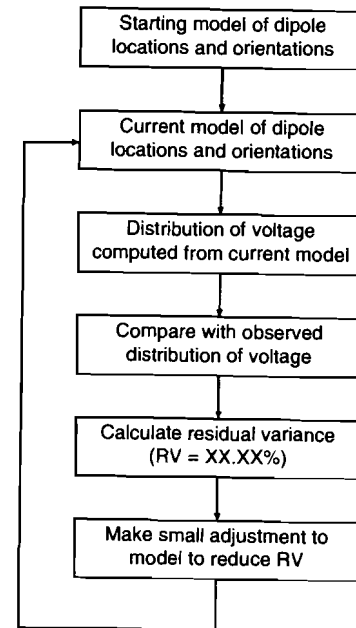
Figure 7.1 Basic procedure of the BESA technique.
