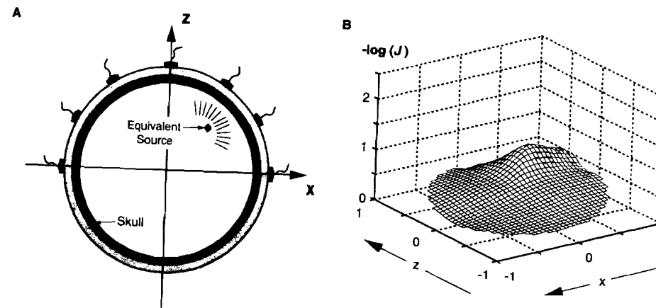
Figure 7.5 Example of a distributed electrical source (A) and the amount of error that would occur in estimating this source by a single dipole over a range of positions (B). Although a single point of minimum error exists, the amount of error varies little over a fairly wide range. (Adapted from Koles, 1998. © 1998 Elsevier Science Ireland Ltd.) Thanks to Zoltan Koles for providing electronic versions of these images.
