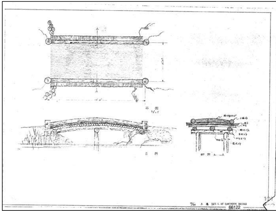
Detail of Earthen Bridge, Japanese Tea Garden, University of Washington, 1959
