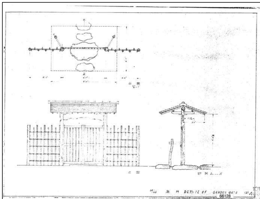
Detail of Garden Gate (2), Japanese Tea Garden, University of Washington, 1959
