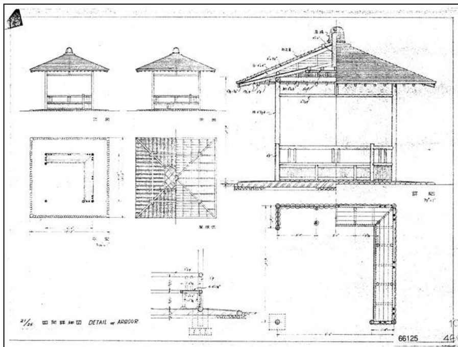
Detail of Arbour, Japanese Tea Garden, University of Washington, 1959
