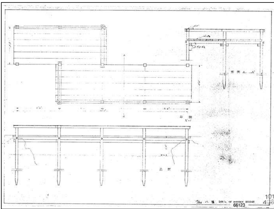
Detail of Wooden Bridge, Japanese Tea Garden, University of Washington, 1959
