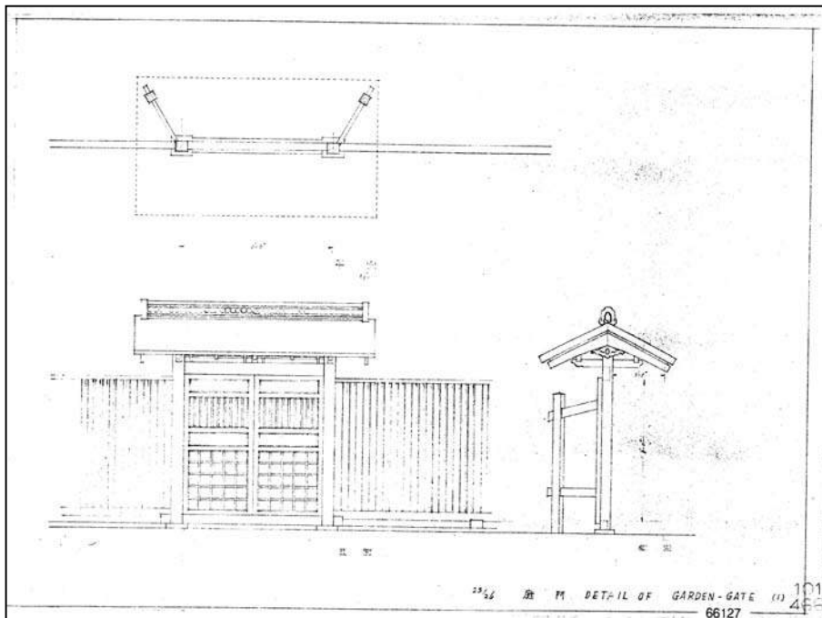
Detail of Garden Gate (1), Japanese Tea Garden, University of Washington, 1959
