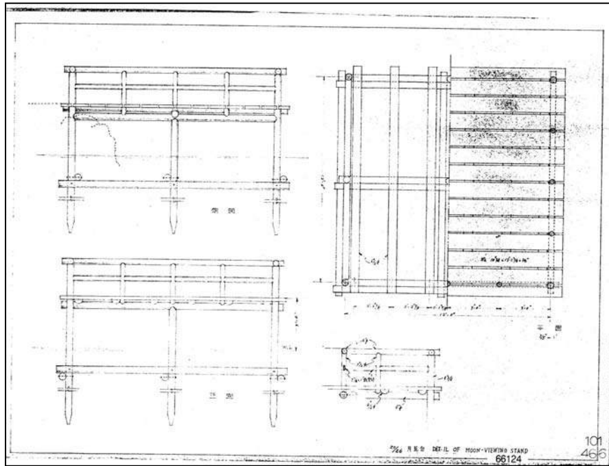
Detail of Moon Viewing Stand, Japanese Tea Garden, University of Washington, 1959
