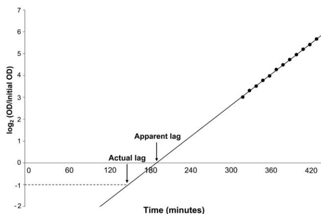
Figure 2. Schematic illustration showing how the apparent duration of lag phase is corrected for freeze-thaw (FT) survival to calculate the actual duration of the physiological lag before growth. The apparent duration is calculated by extrapolating the regression line based on exponential growth back to the initial optical density. In this hypothetical example, 50% of the cells survived the FT treatment; therefore, the initial density of viable cells is half that implied by the initial optical density ( \log_2 0.5 = -1 ). The actual duration of the physiological lag is then obtained by extending the extrapolated growth trajectory until it intersects the initial density of viable cells.
