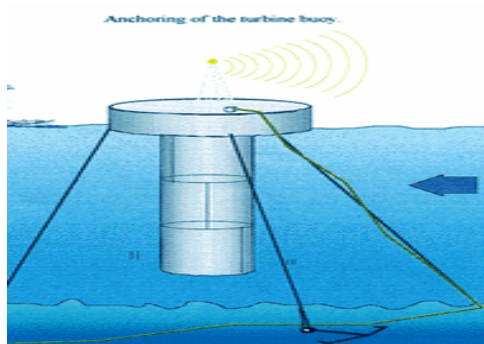
Figure 9. Seapower Vertical Axis Turbine
