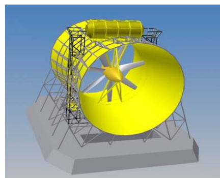
Figure 5. Lunar Energy RTT Turbine
