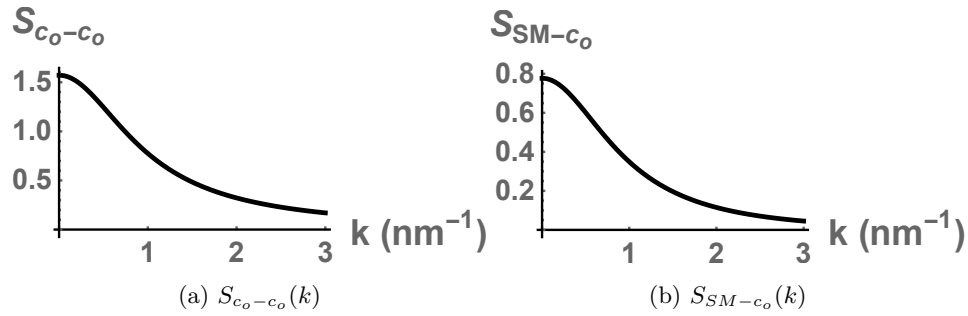
Figure 4: Two of the structure functions characterizing the outer leaflet
