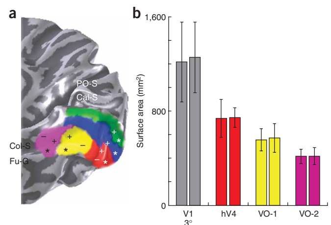
Figure 8 Summary of hV4, VO-1 and VO-2 field map properties. (a) The positions of the ventral-occipital visual field maps V2v (green, 0–16°), V3v (blue, 0–16°), hV4 (red), VO-1 (yellow) and VO-2 (magenta) are shown. The + and – indicate upper and lower visual field representations, respectively. The asterisk indicates the most central visual field representation within each map. PO-S: parietal-occipital sulcus. Cal-S: calcarine sulcus. Col-S: collateral sulcus. Fu-G: fusiform gyrus. (b) The surface area of each map was defined by a 3° expanding ring stimulus and measured along the cortical manifold. The left and right hemispheres correspond to the left and right bars. Error bars: \pm 1 s.d.
