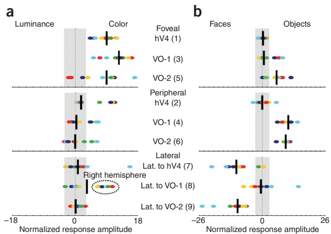
Figure 7 Stimulus selectivity measurements. The normalized response amplitudes in nine ROIs during the color-luminance (a) and object-face (b) experiments are shown. The top and middle panels show the responses in the central (1,3,5) and peripheral (2,4,6) ROIs (numbers in parentheses indicate ROI numbers; see Fig. 6 ). The bottom panel shows the responses in the three regions lateral to the maps (7,8,9). The circles represent the normalized responses for individual subjects ( n = 5 , two hemispheres per subject) and are colored by subject. The dark vertical bars represent the median response. The shaded regions represent a significance level P > 0.001 (uncorrected). The dotted oval indicates measurements from the right hemisphere. Subjects S1, S2, S4, S5, S6.
