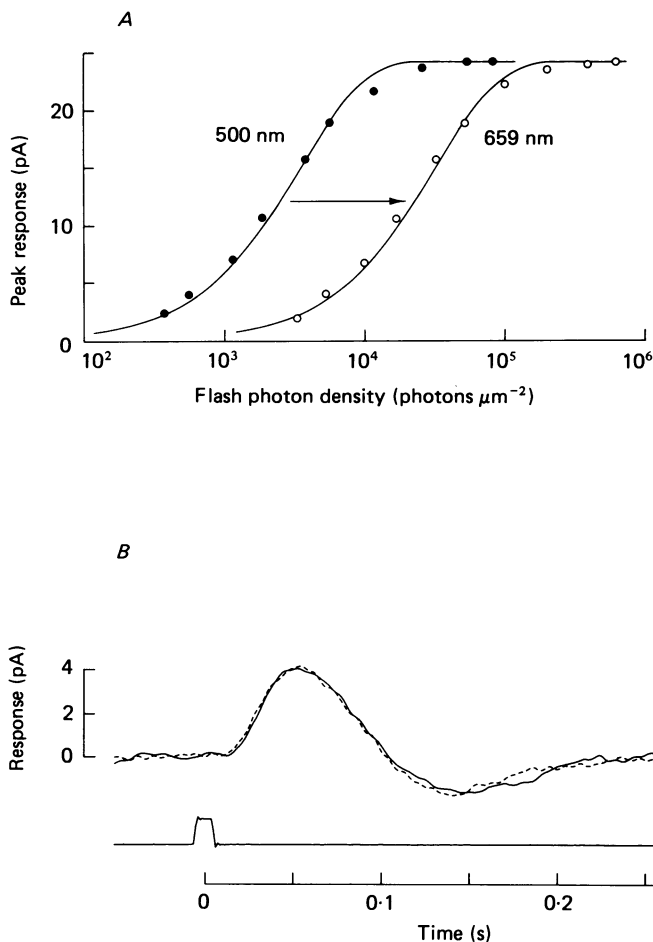
Fig. 2. A , relation between peak response amplitude and flash photon density for the families illustrated in Fig. 1. ●, 500 nm; ○, 659 nm. Smooth curves drawn according to eqn. (5) with k = 2.77 \times 10^{-4} photons ^{-1} \mu\text{m}^2 at 500 nm, and 3.01 \times 10^{-5} photons ^{-1} \mu\text{m}^2 at 659 nm. Light was unpolarized. B , responses at 500 nm (continuous curve) and 659 nm (dashed curve) after adjusting flash strength to equate photon capture. Flash strength in photons \mu\text{m}^{-2} (and number of responses comprising the average) was 574 (17), and 5360 (13) at 500 and 659 nm, respectively.
