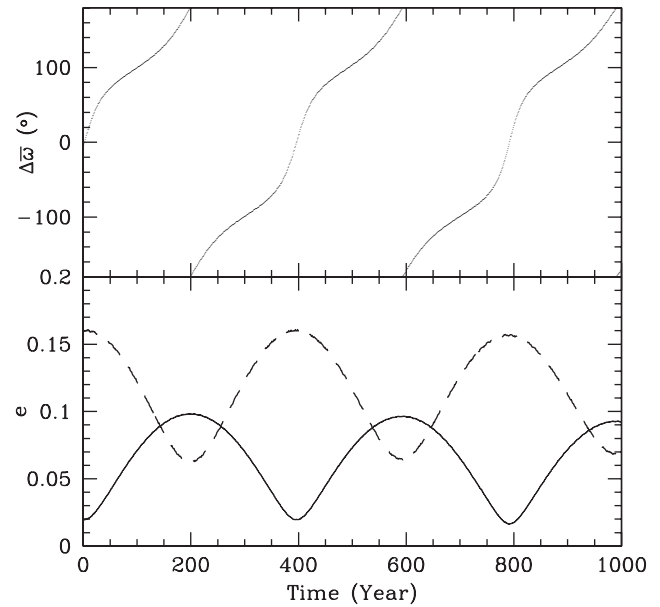
FIG. 8. Apsidal evolution of the Gl 581 b and c planets, see Table 1. Top: The apsidal oscillation is circulation. Bottom: Evolution of e_b (solid line) and e_c (dashed line). The orbits are currently near the extrema of their eccentricity values.
