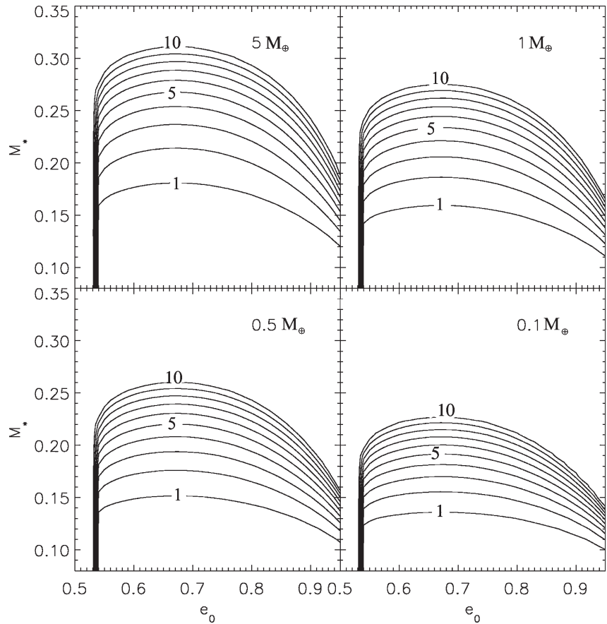
FIG. 2. Contours of \tau_{HL} (in Gyr) represent terrestrial planets that begin at the inner edge of the 0% cloud cover EHZ, as a function of stellar mass and initial eccentricity e_0 . The terrestrial planets have a mass of 5 M_{\oplus} (top left), 1 M_{\oplus} (top right), 0.5 M_{\oplus} (bottom left), and 0.1 M_{\oplus} (bottom right), and a radius determined by Eq. 5. Planets with initial eccentricities below 0.53, or orbiting stars with a mass greater than 0.35 M_{\odot} , are habitable for at least 10 Gyr. Lower-mass planets tend to have longer habitable lifetimes.
