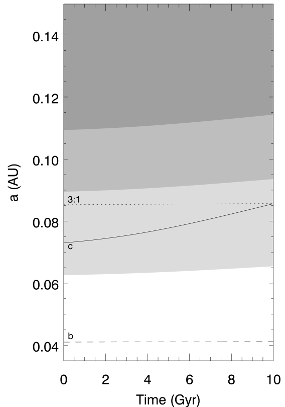
FIG. 10. Evolution of planets b (short-dashed line) and c (solid line) and the instantaneous location of b’s outer 3:1 mean motion resonance (dotted line) for Q_b = 10^6 ; R_b = 3.74 R_\oplus ; k = 3/2 and Q_c = 100 ; R_c = 1.8 R_\oplus ; k = 0.3 . In our model, this evolution is the most plausible, as it prevents planet c from crossing the 3:1 mean-motion resonance and reaching the 50% cloud cover habitable zone (medium grey). Our calculations predict that this evolutionary history would have permitted stable interactions 10 Gyr ago.
