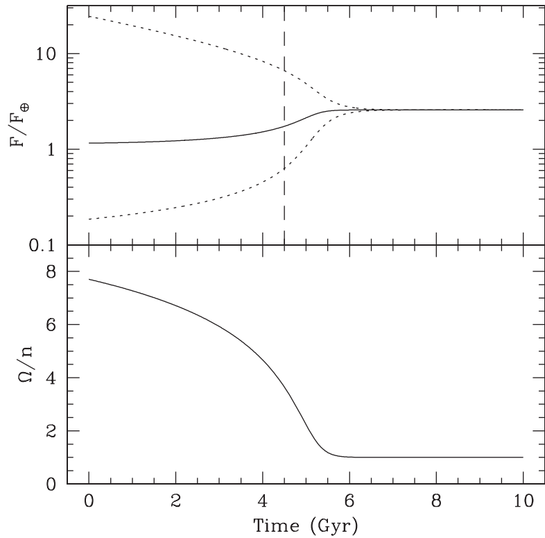
FIG. 4. Top: Orbit-averaged stellar flux received by a tidally evolving planet relative to that of Earth F_{\oplus} (solid line), see Eq. 7, as well as at periastron and apoastron (dotted lines). The planet orbits a 0.2 M_{\oplus} star with initial orbital elements of a_0 = 0.0877 and e_0 = 0.84 . The tidal lifetime of the planet, 4.5 Gyr in this case, corresponds to the age of Earth and is shown by the dashed line. Note, however, the extreme difference between flux at periastron and apoastron (a factor of 200). Bottom: Ratio of the rotation frequency of the tidally evolving planet to its instantaneous mean motion, cf. Eq. 3. Initially, the planet rotates nearly 10 times faster than it revolves, but after \sim 6 Gyr, the orbit has circularized and \Omega = n .
