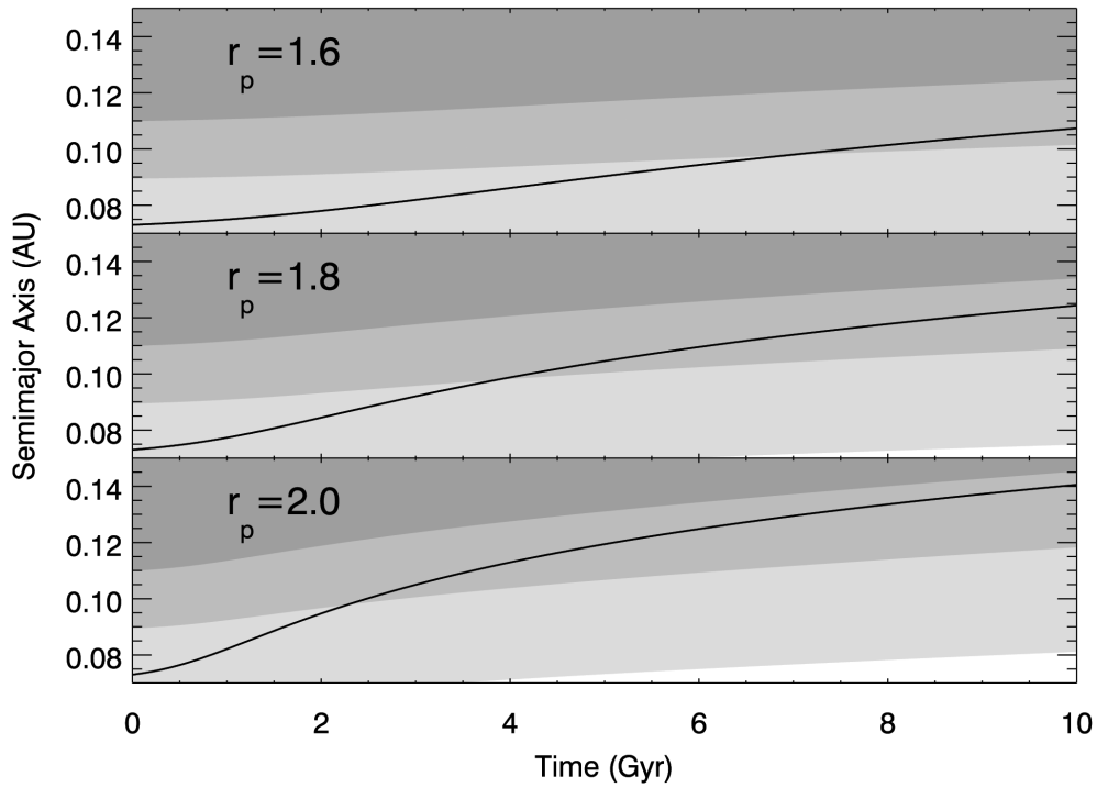
FIG. 6. Evolution of Gl 581 c for three different possible radius values. The shading represents different definitions of the HZ, cf. Fig. 1.
