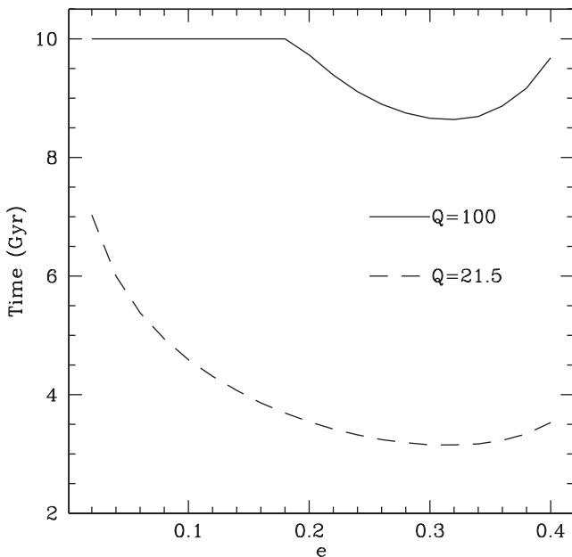
FIG. 5. Time since Gl 581 c would have been habitable as a function of its current eccentricity. We set R_c = 1.8 R_{\oplus} , and consider Q values of 100 and 21.5. The Q = 21.5 case permits habitability as recently as 3 Gyr ago.
