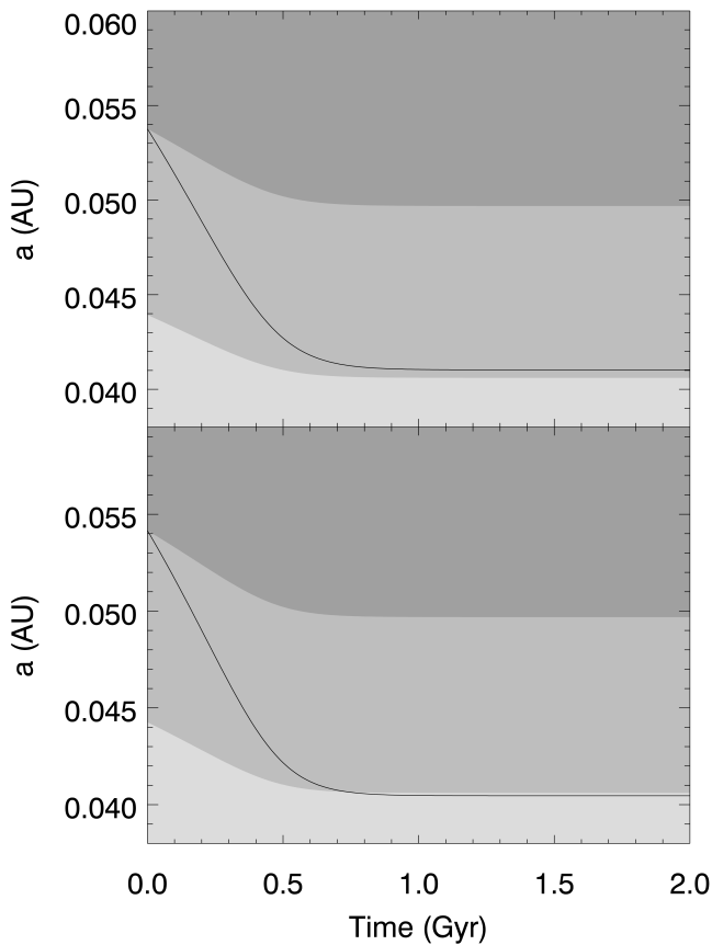
FIG. 3. Evolution of the semi-major axes (solid line) for the orbits of 2 hypothetical planets relative to EHZ boundaries (shown by the shading, cf. Fig. 1). These planets are in orbit about a 0.15 M_{\odot} star. Top: Evolution of a planet with e_0 = 0.52 . This planet’s semi-major orbital axis decreases until its eccentricity reaches zero after 750 million years, at which point the tidal evolution effectively stops. The tidal evolution stops just before the planet crosses the inner edge of the EHZ, and therefore the planet will be habitable indefinitely. Bottom: Evolution of the semi-major axes of a planet with e_0 = 0.54 . Although very similar to the other planet’s evolution, this planet’s larger initial eccentricity results in more torque so that when e reaches zero, the planet is just interior to the 50% cloud cover HZ. The habitable lifetime for this planet is 7.5 \times 10^8 years.
