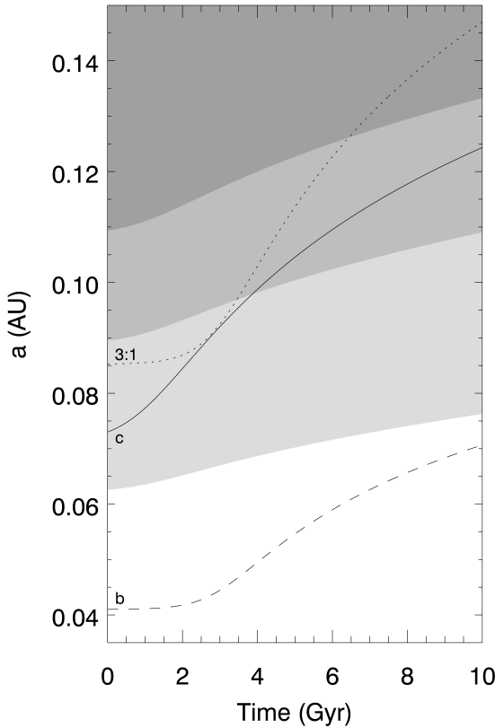
FIG. 9. Evolution of planets b (dashed line) and c (solid line) and the instantaneous location of b’s outer 3:1 mean motion resonance (dotted line) for Q_b = 4 \times 10^4 ; k = 3/2 . In this case, planet c would have just avoided the 3:1 resonance. The shading corresponds to different definitions of the HZ, cf. Fig. 1. Our calculations indicate that 10 Gyr ago the configuration would have been unstable.
