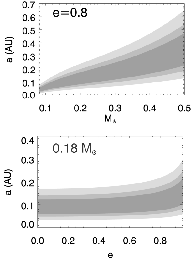
FIG. 1. Semi-major axes illustrate habitability as a function of stellar mass and eccentricity, as calculated from Eqs. 8–11. The shading represents different choices of cloud cover for the limits of the HZ. Darkest gray assumes no cloud cover, medium gray assumes 50% cloud cover, light gray assumes total cloud cover, and white is uninhabitable.
