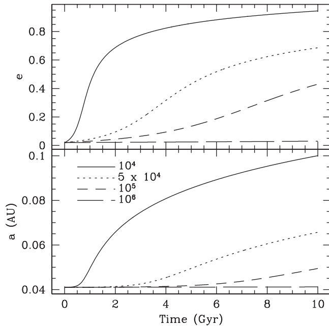
FIG. 7. Evolution of a_b and e_b for various choices of Q_b , assuming k = 3/2 . The evolution is negligible unless Q_b \leq 10^5 .
