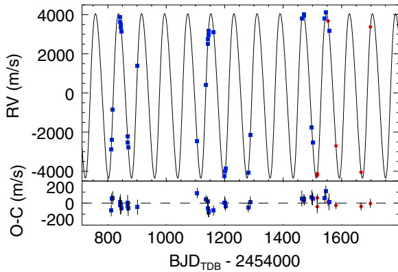
Figure 4. Derived relative radial velocities from the MARVELS (blue squares) and SARG (red circles) spectrographs are overlaid with the best-fit orbital solution described in Section 4 and compiled in Table 3. Residuals to this fit are shown in the bottom panel.
