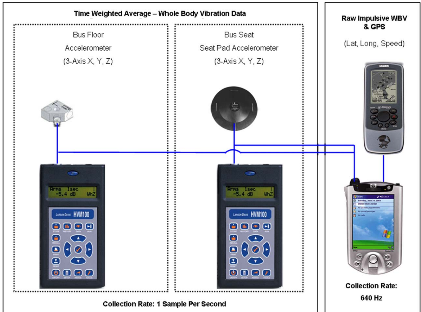
Fig. 2. Schematic of WBV Data Collection System.
