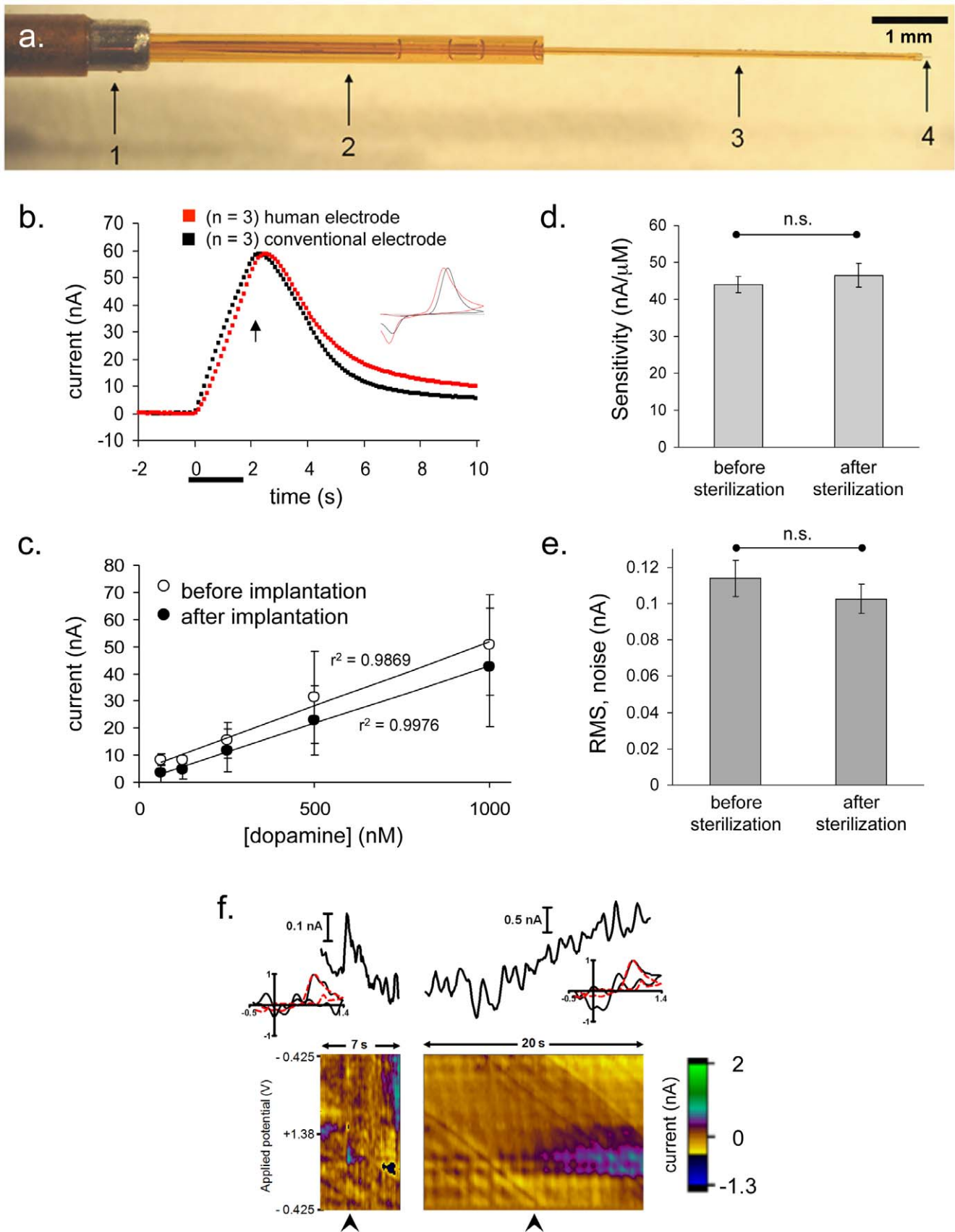
Figure 1. Human-compatible carbon fiber microelectrode can detect dopamine in human striatum. (a) Human electrode assembly comprised of protective tube with reference electrode at the tip (1), large-gauge fused silica capillary (2), small-gauge fused silica (3) and carbon fiber (4). (b) Average change in peak oxidative current in rat striatum following electrical stimulation (60 Hz, 120 pulses, 300 \mu A) of dopamine axon
