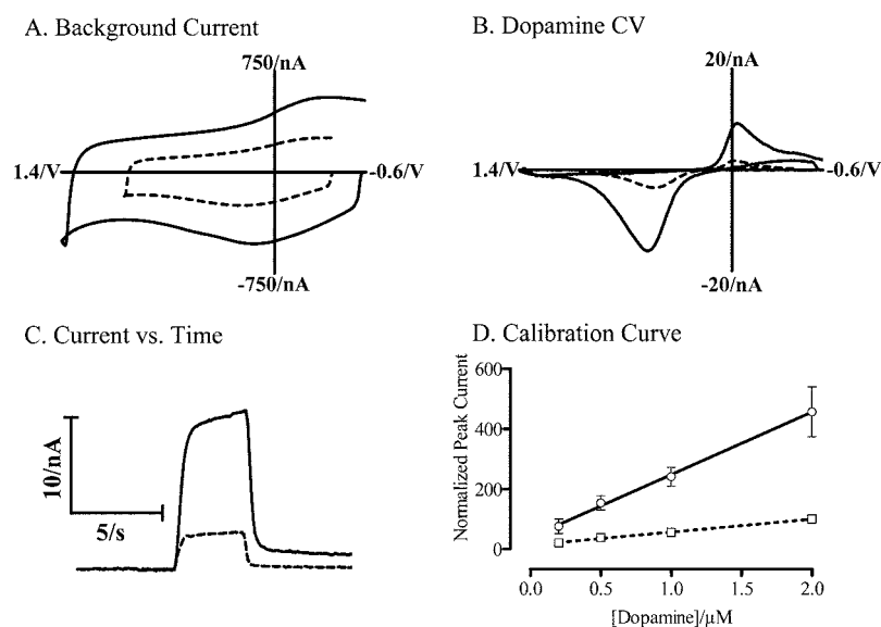
Fig. 1 In vitro characterization of waveforms. The traditional waveform ( -0.4 V to 1.0 V, 300 \text{ V s}^{-1} ) is shown in dashed lines, while the extended waveform ( -0.6 V to 1.4 V, 400 \text{ V s}^{-1} ) is shown in solid lines. A: Background cyclic voltammograms for the two potential limits at the same electrode recorded in TRIS buffer solution, pH 7.4. B: Background-subtracted cyclic voltammograms for 1 \mu\text{M} dopamine. C: Response to a bolus dopamine injection, in which the peak oxidation current of each cyclic voltammogram is plotted vs. time. D: Calibration curve for dopamine ( n = 6 ). Due to variations between electrodes, each electrode response was normalized to the response for 2 \mu\text{M} dopamine with the traditional waveform. The error bars represent the standard deviation.
