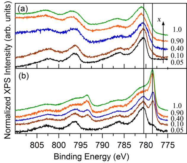
FIG. 3 (color online). (a) Normalized Co 2p XPS data for x = 0.05 (black), 0.10 (brown), 0.40 (blue), 0.90 (orange), and 1.00 (green) \text{Zn}_{1-x}\text{Co}_x\text{O} crystallites collected without sputtering. The \text{Co}^{2+} 2p_{3/2} and 2p_{1/2} peaks shift to higher binding energies with increasing x . The lines at 778.5 and 780.7 eV are guides to the eye. The spectra are normalized to the \text{Co}^{2+} 2p_{3/2} intensity at 781 eV and offset for clarity. (b) Spectra of the same series of samples collected after \text{Ar}^+ sputtering, showing increasing \text{Co}^0 intensity with increasing x (sharp peaks at 778.5 and 793.5 eV). The \text{Co}^0 intensity is an artifact of the \text{Ar}^+ sputtering process, which itself causes reduction of \text{Co}^{2+} to form \text{Co}^0 .
