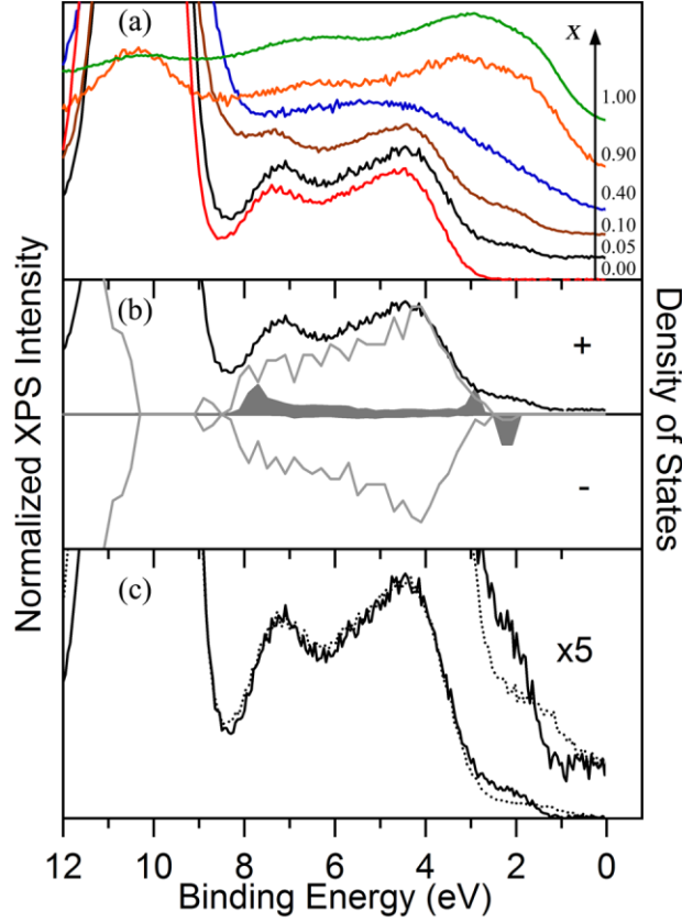
FIG. 2 (color online). XPS data for the valence band and Zn 3d region of \text{Zn}_{1-x}\text{Co}_x\text{O} crystallites. (a) Data for x = 0.00 (red), 0.05 (black), 0.10 (brown), 0.40 (blue), 0.90 (orange), and 1.00 (green) samples, normalized to the O 2p peak maximum and offset for clarity. (b) Comparison of the valence band XPS spectrum for x = 0.05 (black) with the spin-resolved total density of states (grey) and \text{Co}^{2+} partial density of states (filled, \times 10 ) calculated by density functional theory for x = 0.006 (adapted from ref. 27). The increasing intensity above the top of the ZnO valence band with increasing x is due to occupied \text{Co}^{2+} 3d levels. (c) XPS spectrum for x = 0.05 (solid curve) and sum of the XPS spectra for x = 0.00 and x = 1.00 weighted to yield x_{\text{avg}} \sim 0.05 (dotted line, x_{\text{loc}} \sim 1.0 ).
