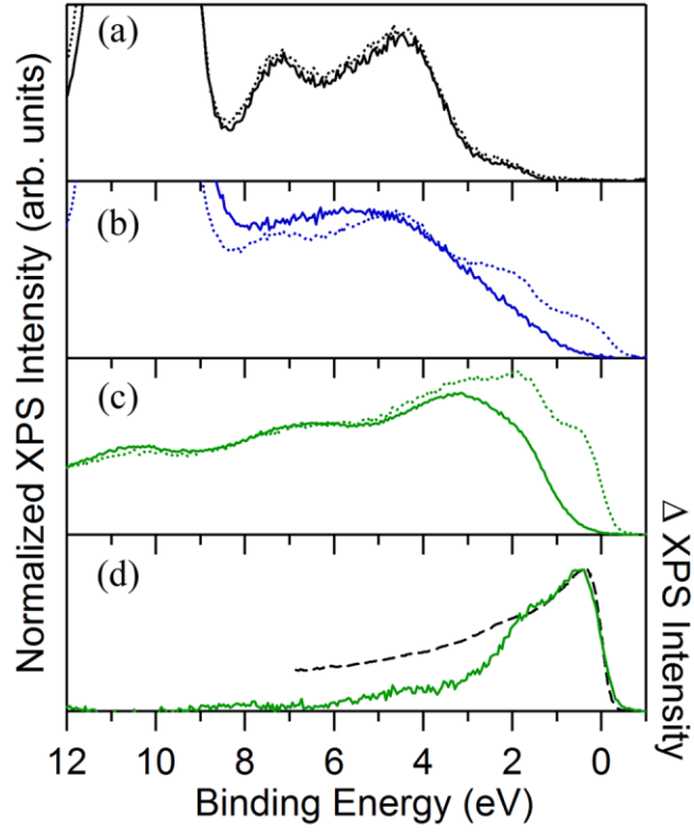
FIG. 4 (color online). Normalized valence band XPS spectra collected before (solid) and after (dotted) sputtering for x = (a) 0.05, (b) 0.40, and (c) 1.0 \text{Zn}_{1-x}\text{Co}_x\text{O} crystallites. (d) The difference between before and after sputtering for the x = 1.0 sample (green solid), and an experimental \text{Co}^0 XPS spectrum (black dashed, adapted from ref. 34). The \text{Co}^0 intensity is an artifact of the \text{Ar}^+ sputtering process, which itself causes reduction of \text{Co}^{2+} to form \text{Co}^0 .
