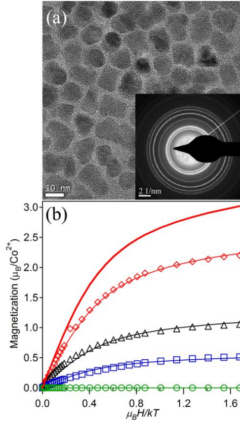
FIG. 1 (color online). (a) TEM image of x = 1.00 (w-CoO) nanocrystals. The scale bar is 10 nm. The electron diffraction pattern shown in the inset reveals the wurtzite structure of these nanocrystals. (b) 2K magnetization for x = 0.0075 (red diamonds), 0.05 (black triangles), 0.40 (blue squares), and 1.00 (green circles) samples (data adapted from ref. 16). The solid lines show calculated 2K powder magnetization curves for paramagnetic \text{Co}^{2+} in the wurtzite lattice structure at different values of x_{\text{eff}} , as described in the text.
