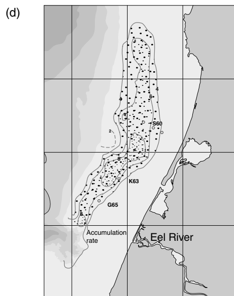
after Sommerfield and Nittrouer, 1999
