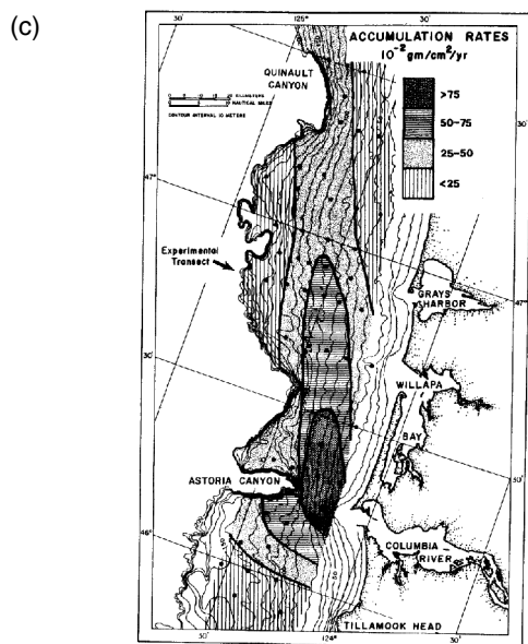
Nittrouer and Sternberg, 1981
