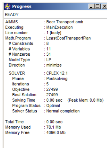
Figure 5.3: The AIMMS progress window
