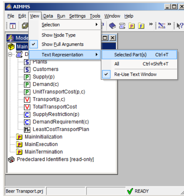
Figure 3.13: View text model
