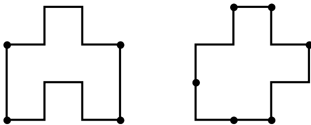
Figure 7. Planigons without center have boundary partitioned into 4 or 6 arcs, such that the opposite arcs are translates of each other.
