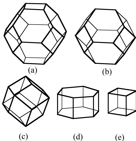
Figure 2. Representatives of the five combinatorial types of convex parallelhedra, as determined by Fedorov [9]. (a) is the truncated octahedron (an Archimedean polyhedron); (b) is an elongated dodecahedron (with regular faces, but not Archimedean); (c) is Kepler's rhombic dodecahedron K (a Catalan polyhedron); (d) is the Archimedean 6-sided prism; and (e) is the cube.
