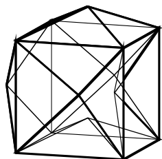
Figure 15. A mono-hedral parallelohedron with triangles as faces.
