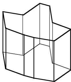
Figure 14. A non-convex parallelohedron without a center of symmetry.
