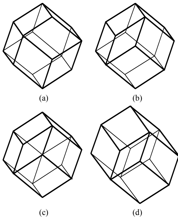
Figure 9. Indentations of the Kepler rhombic dodecahedron K, shown in (a). In (b) is presented the indentation at the vertex nearest to the observer; this is the only indentation arising from (a). A double indentation of the dodecahedron in (a), which is a single indentation of (b), is shown in (c); it fails to be a polyhedron of the spherical type, since two distinct vertices coincide at the center; hence it is not admitted. By stretching one of the zones, as in (d), an admissible polyhedron is obtained — but it is not a rhombic monohedron.
