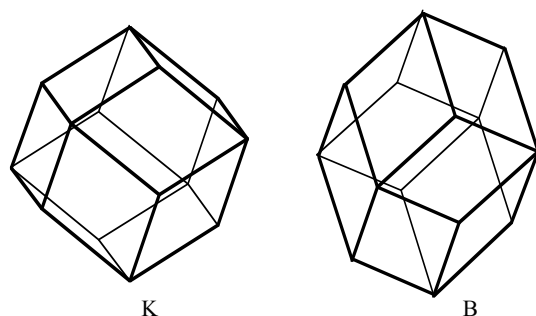
Figure 3. The two convex rhombic monohedra (isozonohedra): Kepler's K and Bilinski's B.
