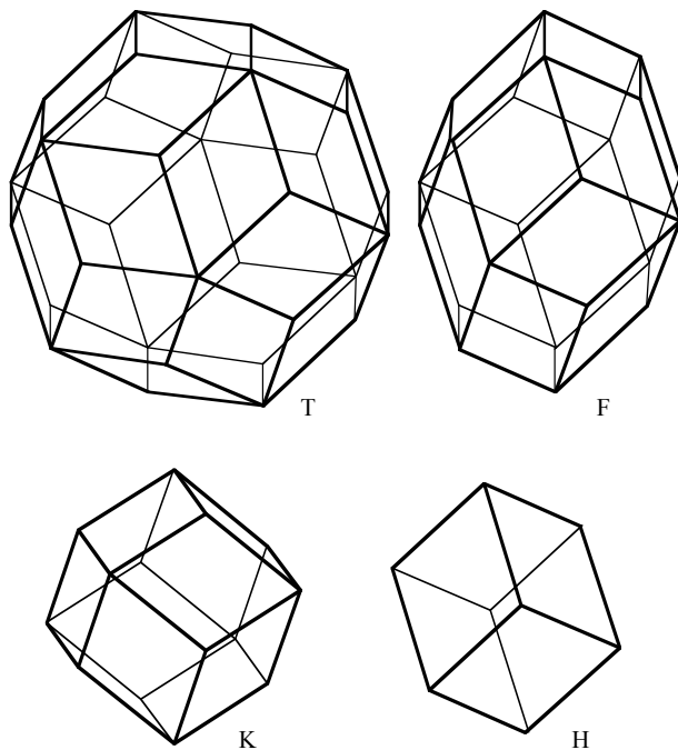
Figure 1. The four isozonohedra (convex rhombic monohedra) enumerated by Fedorov. Kepler found the triacontahedron T and the dodecahedron K, while Fedorov discovered the icosahedron F. The infinite class H of rhombic hexahedra seems to have been known much earlier.
