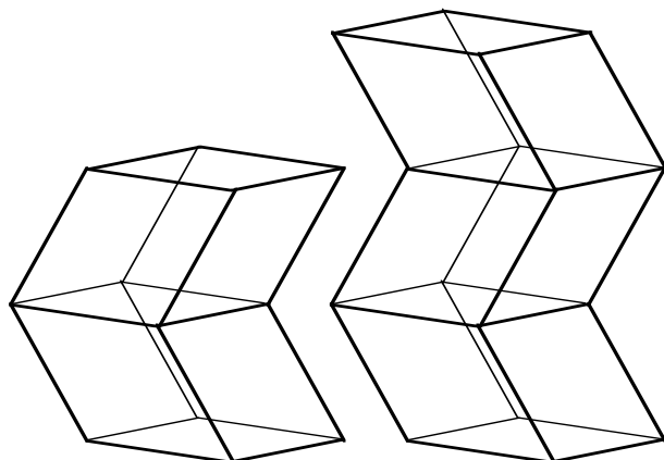
Figure 13. Isozonohedra with 10 and 14 faces.
