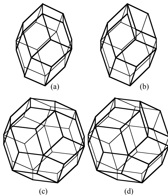
Figure 11. (a) Icosahedron F and (b) its indentation; (c) Triacantahedron T and (d) its indentation.
