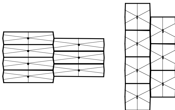
Figure 6. An affine transform of the lattice of centers at left leads to the lattice of the tiling by regular hexagons. The Dirichlet domains of the points of the lattice are transformed into the hexagons at right, which clearly are not affinely equivalent to regular hexagons.
