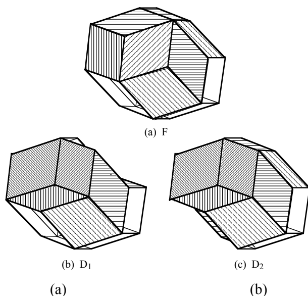
Figure 12. (a) The Fedorov rhombic icosahedron F ; (b) A double indentation of the F yields a non-convex rhombic icosahedron D_1 of the spherical type that is a parallelohedron; (c) A different double indentation D_2 is also a parallelohedron.
