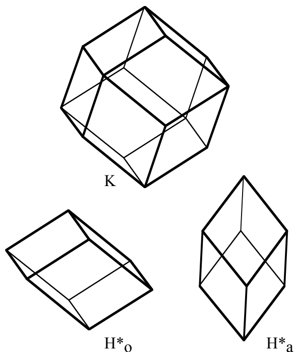
Figure 5. Kepler's rhombic dodecahedron K and its descendant, rhombohedron H^*_o . The rhombohedron H^*_a is "related" to them since its faces are congruent to those of the other two isozonohedra shown; however, it is not obtainable from K by zone elimination.
