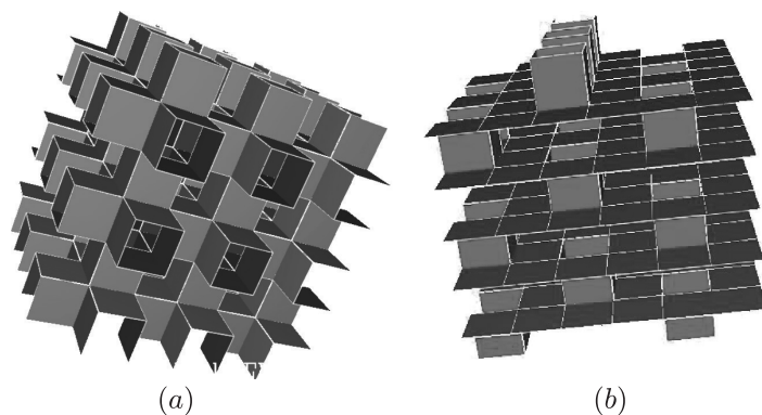
Fig. 16. (a) An isotropic sponge (4.4.4.4.4) with incidence symbol (a \hat{a} a \hat{a} a \hat{a} \hat{a}; a) . This is one of the three regular Coxeter–Petrie sponges; all are isotropic. (b) A layered sponge (4.4.4.4.4) with incidence symbol (a^+ b^+ c^+ d^+ e^+; a^- b^- c^- d^+ e^-)
