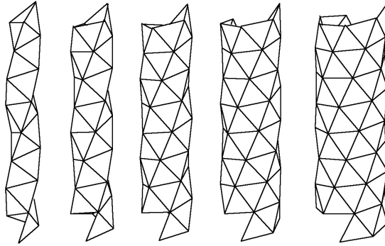
Fig. 9. Acoptic helical rods. In the notation explained in Fig. 10, they can be described by (1, m, m + 1) , for m = 2, 3, 4, 5, 6
