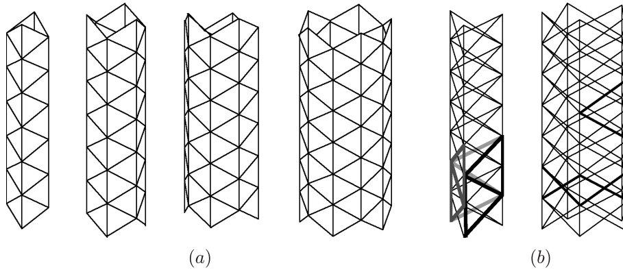
Fig. 5. (a) Acoptic unary ribboned rods R(3.3.3.3.3.3)_n , for n = 4, 6, 8, 10 . (b) Unary ribboned rods R(3.3.3.3.3.3)_3 and R(3.3.3.3.3.3)_5
