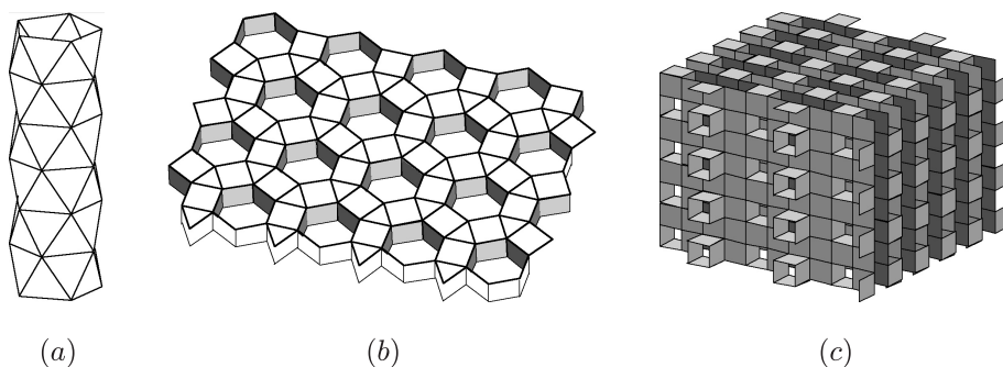
Fig. 1. (a) A rod with vertex symbol (3^6) . (b) A slab with vertex symbol (3.4^4) . (c) A sponge with vertex symbol (4^5)
