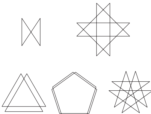
Fig. 8. Isogonal polygons with ratio of sides \sqrt{3}/2 = 0.866\dots . These are cross-sections of binary ribbons R(3.3.3.4.4)_n with n = 4/2, 8/3, 6/2, 10/2, 10/3 , respectively
