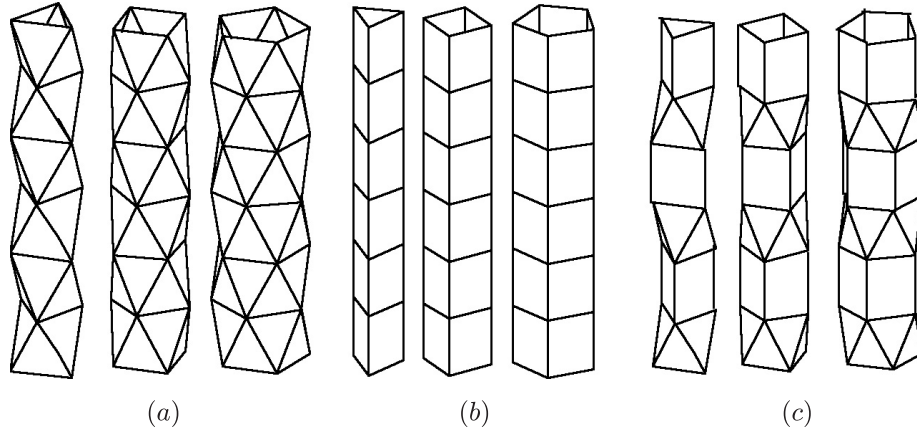
Fig. 3. Uniform acoptic stacked rods with \{n\} bases, n = 3, 4, 5 . (a) Unary triangle-faced rods (3.3.3.3.3.3)_n . (b) Unary square-faced rods (4.4.4.4)_n . (c) Binary rods (3.3.3.4.4)_n
