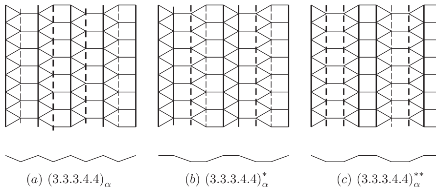
Fig. 13. The three corrugations that arise from (3.3.3.4.4) (and also from (3.3.3. - 4. - 4)). (a) The angle of bend satisfies 0 < \alpha < \pi/2 . (b) Here 0 < \alpha < \pi ; note that for \alpha \geq 115.66^\circ the slab is selfintersecting. (c) Here 0 < \alpha < \pi as well; note that for \alpha \geq 125.26^\circ the slab is selfintersecting
