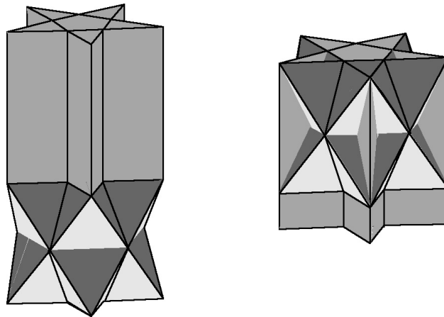
Fig. 4. Two possible pairs of modules with \{5/2\} bases, leading to binary stacked rods that can be denoted (3.3.3.4.4)_{5/2} and (3.3.3. - 4. - 4)_{5/2} , respectively. Notice that in the latter rod there are several simultaneous overlaps of squares. There are four other binary stacked rods with pentagrammatic bases: (3.3.3.4.4)_{5/3} and (3.3.3. - 4. - 4)_{5/3} , (3.3.3.3.3.)_{5/2,5/3} and (3.3.3. - 3. - 3. - 3)_{5/2,5/3}
