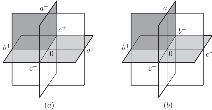
Fig. 19. The two labeled vertex stars ( 4^5 ) possible in the cubic lattice. (a) Asymmetric vertex star label a^+b^+c^+d^+e^+ . (b) Symmetric vertex star label a^+b^+c^+c^-b^- , using the mirror that contains the Oa edge and bisects the angle c^+Oc^- . Other symmetries that a vertex star may possess lead to other vertex star labels
