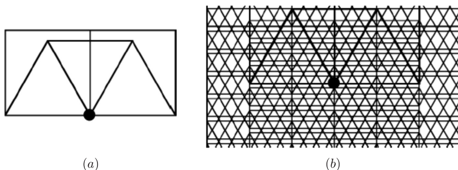
Fig. 11. The non-acoptic uniform tiling (3.3.3. – 4. – 4). (a) The vertex star. (b) A patch of the tiling, illustrating the multiple overlaps of the tiles
