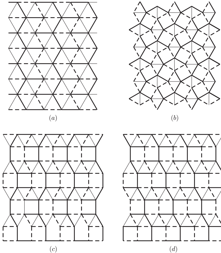
Fig. 14. The four parametrized families of crinkles. (a) (3.3.3.3.3.3)_\alpha^\# ; (b) (3.3.4.3.4)_\alpha^\# ; (c) (3.3.3.4.4)_\alpha^\# ; (d) (3.3.3.4.4)_\alpha^{\#\#} , where \alpha denotes the angle of the bend. For \alpha \rightarrow 0 each tends to the corresponding tiling. If \alpha \rightarrow \pi , the crinkle (3.3.3.3.3.3)_\alpha^\# has a discontinuity: (3.3.3.3.3.3)_\alpha^\# is a (2-dimensional) crinkle, while (3.3.3.3.3.3)_\pi^\# is just a strip of triangles. If \alpha \rightarrow \pi , (3.3.4.3.4)_\alpha^\# \rightarrow (3.3.3. - 4. - 4) , which is the tiling illustrated in Fig. 11. The crinkles in (c) and (d) have in fact three different angles of bend; \alpha denotes the bend along edges between triangles. For \alpha \rightarrow \pi , each of these crinkles tends to a non-acoptic structure that is not a uniform polyhedral
