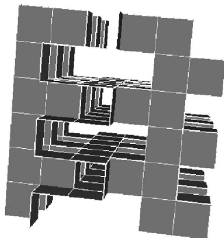
Fig. 17. A uniform sponge (4.4.4.4) = (a^+b^+c^+d^+e^+; a^-b^+c^-d^+e^-) from [10], where it is denoted N1 . Like several other sponges from [10], this is neither isotropic nor layered. It was first described in [14]
