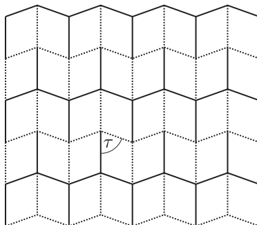
Fig. 22. An isohedral tiling by parallelograms, described by Miura [30]. It can be folded to yield a crinkled slab; heavy solid edges indicate ridges, dashed ones valleys
