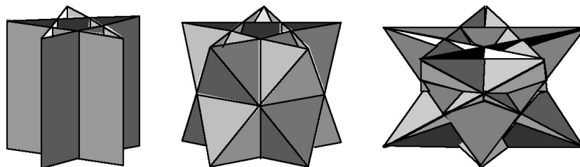
Fig. 2. The pentagram-based prism (4.4.5/2) and antiprisms (3.3.3.5/2) and (3.3.3.5/3)
