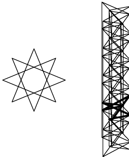
Fig. 6. The ribboned rod R(3.3.3.3.3.3)_{8/3} shown alongside its cross-section
