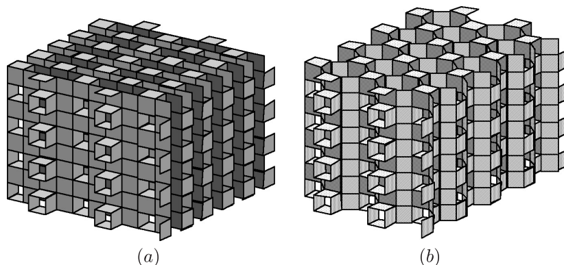
Fig. 21. The sponge in (a) is another view of the sponge in Fig. 16(b). It can be “stretched” (or “flexed”) in a continuous way to yield the one in (b). Both have the same adjacency symbol (a^+b^+c^+d^+e^+; a^-b^-c^-d^+e^-) , hence should be considered as being of the same “type”. The sponge (a) appears in [41] as 4^5(8) , but the sponge (b) is missing from that collection
