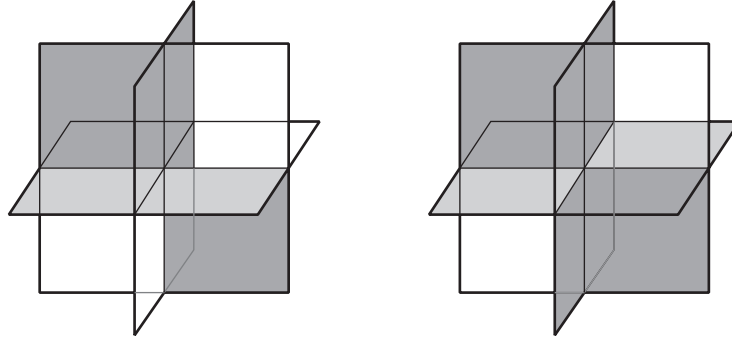
Fig. 20. The two vertex stars associated in the cubic lattice with the vertex symbol (4^6) . Each admits several vertex star labels
