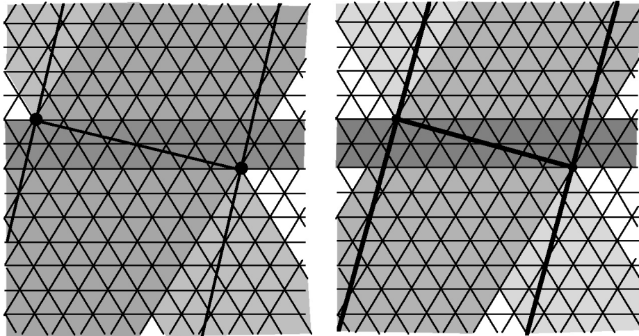
Fig. 10. The construction of the helical rods (1, 4, 5) and (2, 5, 7) . In each case the strip between the parallel heavily drawn lines should be used to generate the rod by making the two heavy dots coincide. The perpendicular to these lines (which becomes an equatorial section of the rod) is intersected by 1, 4, and 5 = 1 + 4 , and by 2, 5, and 7 = 2 + 5 helical strips of triangles, respectively; this explains the notation (1, 4, 5) and (2, 5, 7) for these helical rods. The general acoptic helical rod has symbol of the form (m, n, m + n) , with 1 \leq m < n ; the notation for non-acoptic helical rods is (m, n, m + n)/k if the triangles of the rod form a rod of type (m, n, m + n) , that winds k \geq 1 times about the axis
