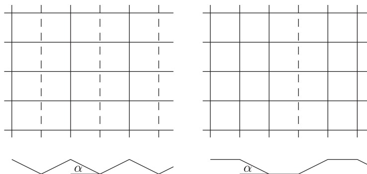
Fig. 12. The two families of corrugated slabs derived from the (4.4.4.4) tiling. (a) Here 0 < \alpha < \pi/2 . (b) Here 0 < \alpha < \pi ; note that for \alpha \geq 2\pi/3 the slab is selfintersecting
