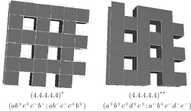
Fig. 15. Two distinct tunneled slabs that cannot be distinguished by their vertex symbols without the asterisks. These slabs, as well as the illustrations in Section 5, were created by Steven Gillispie
