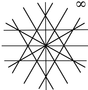
Figure 3: A view of the arrangement \mathcal{A}(13, 1) from the family \mathcal{R}(2) .
